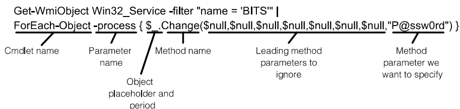
Figure 13.3 Breaking down the ForEach-Object cmdlet
