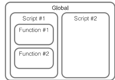
Figure 17.6 Global, script, and function (private) scopes
