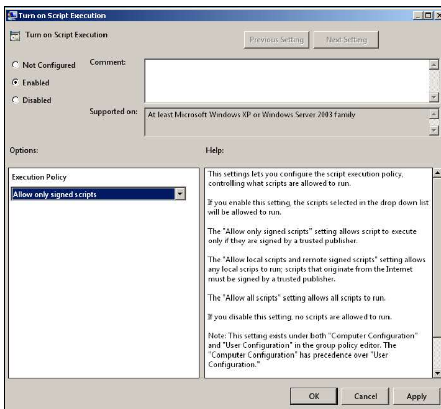
Figure 14.2 Changing the Windows PowerShell execution policy in a Group Policy object
