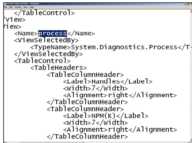
Figure 8.1 Locating the Process view in Windows Notepad
