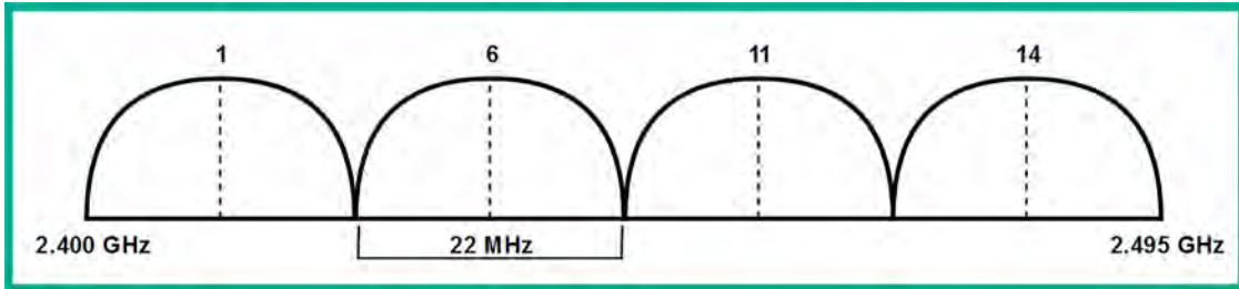
Figure 14.2: Non-overlapping channels
