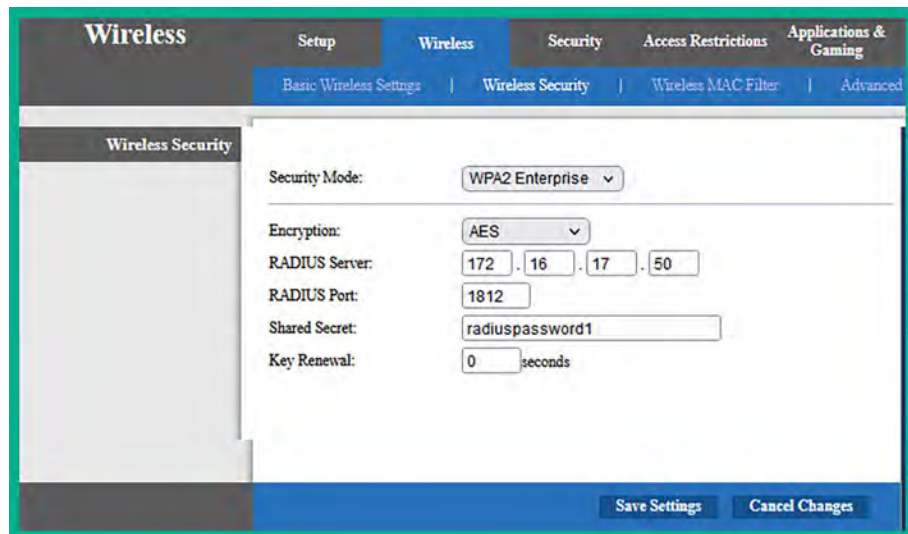
Figure 3.45: Wireless router security configuration
