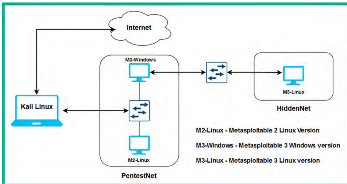
Figure 2.46: Low-level lab diagram
