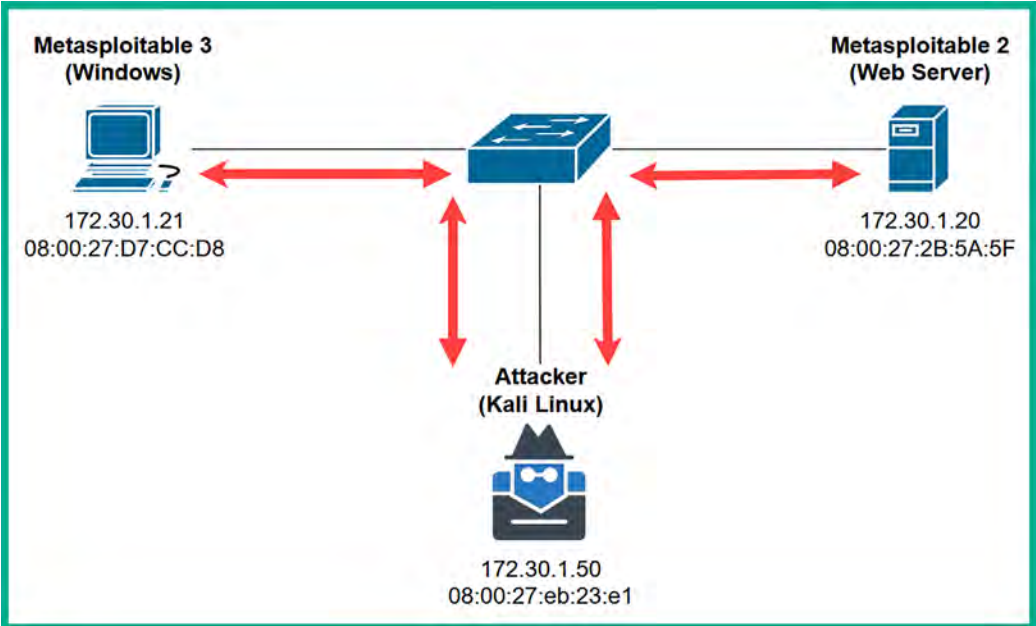
Figure 10.67: MITM
