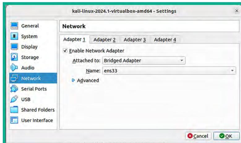
Figure 19.8: Network Adapter 1
