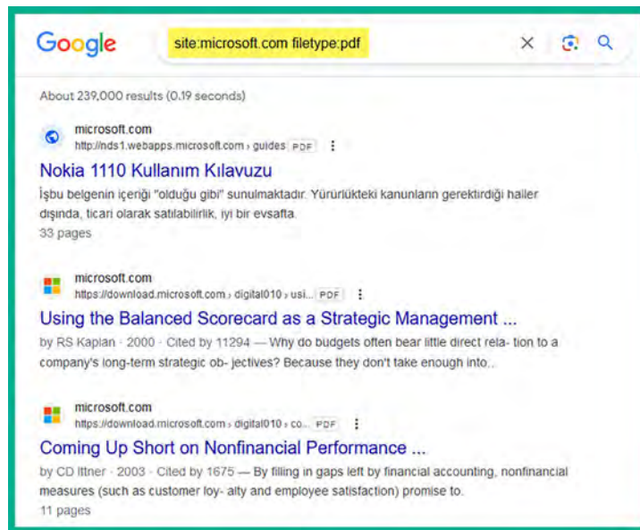
Figure 5.4: Specific filetype
