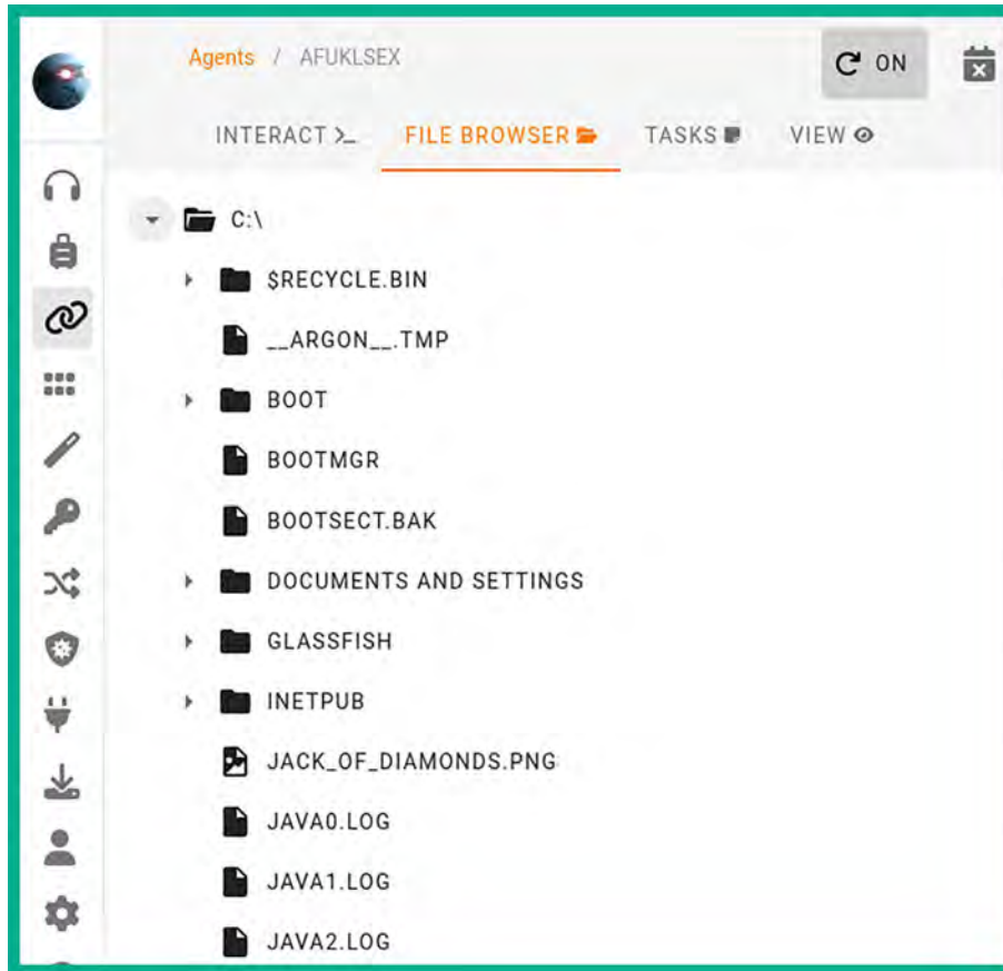
Figure 11.63: File browser
