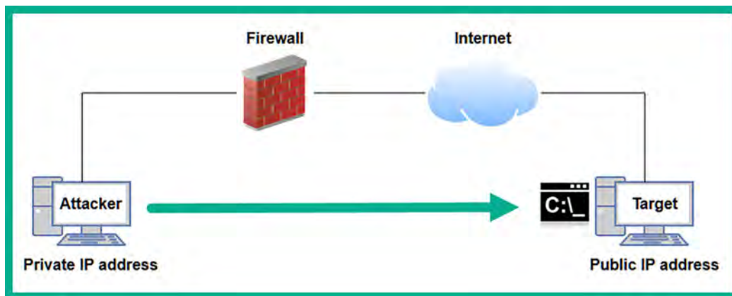
Figure 8.1: Bind shell
