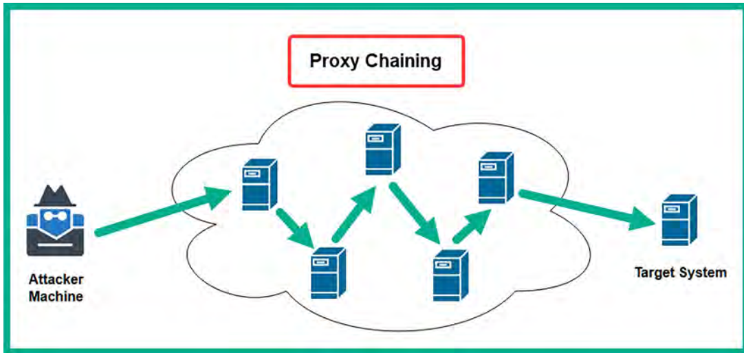
Figure 4.5: Proxy chaining
