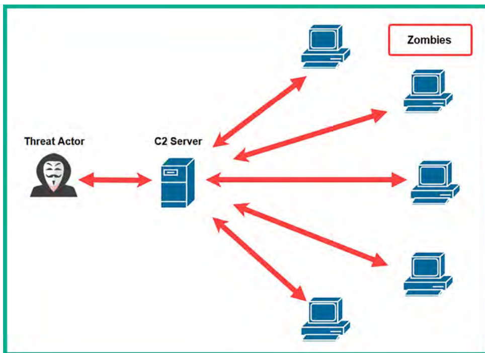
Figure 11.1: C2 operations
