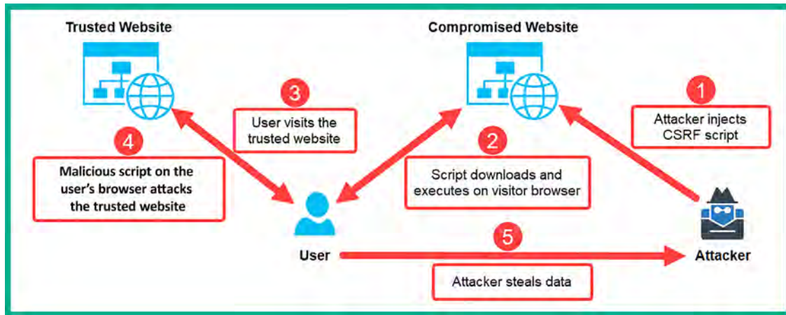
Figure 17.41: CSRF
