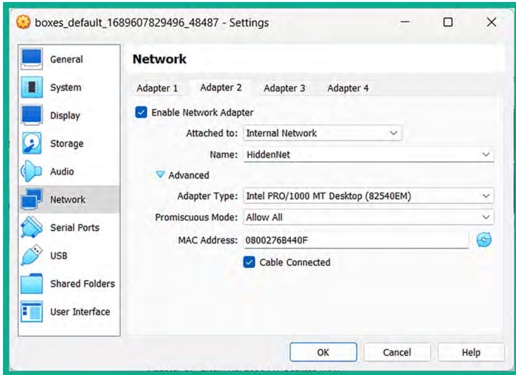
Figure 2.57: Network | Adapter 2
