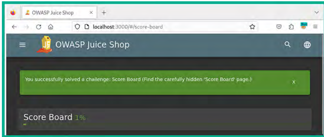
Figure 16.22: Score Board
