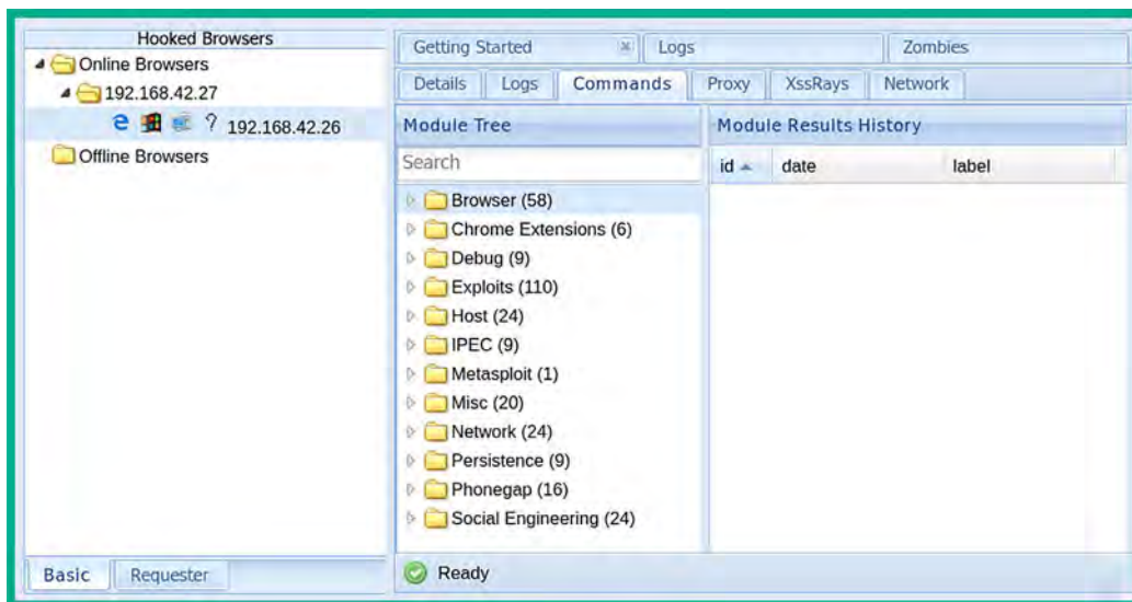
Figure 17.75: BeEF modules
