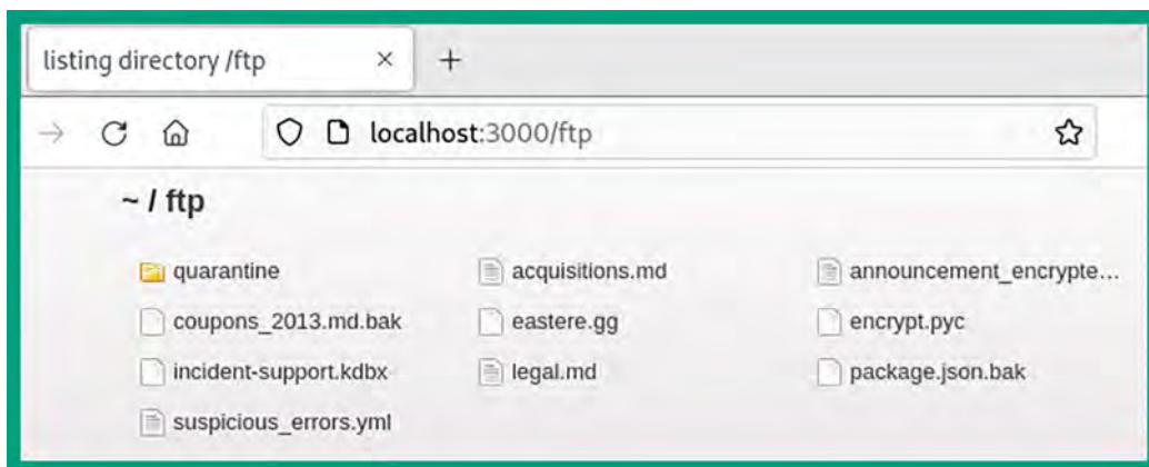
Figure 16.39: Hidden directory
