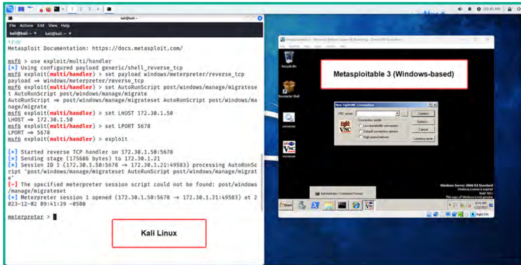
Figure 10.42: Reverse shell
