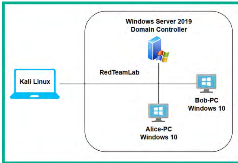
Figure 12.3: Redteamlab topology
