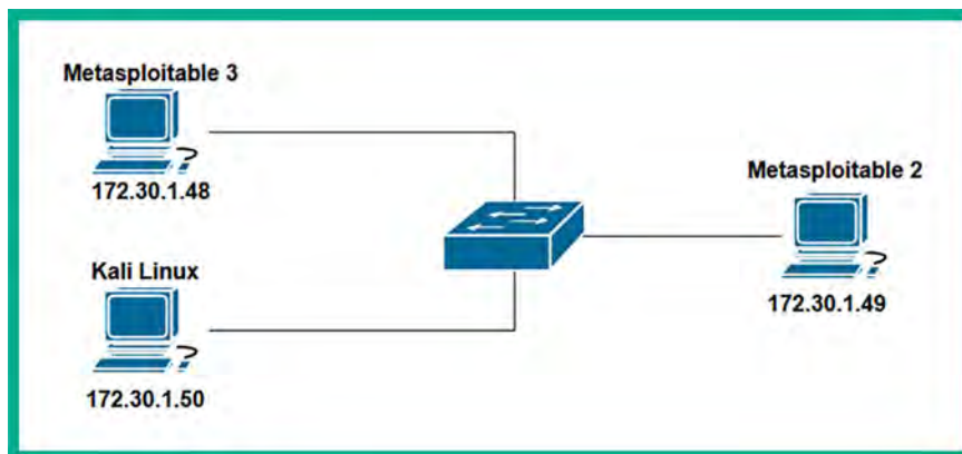
Figure 6.20: Decoys
