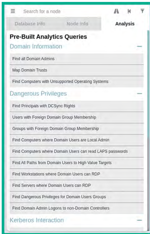
Figure 12.37: Analysis options
