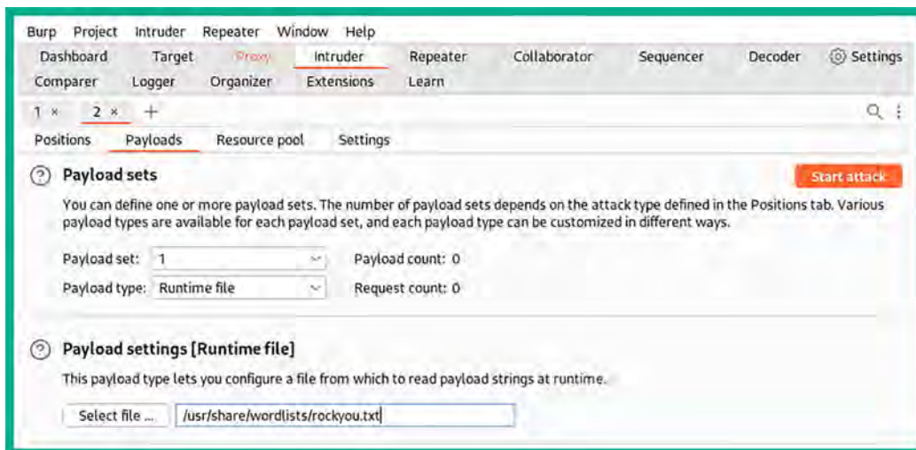
Figure 17.15: Wordlist file
