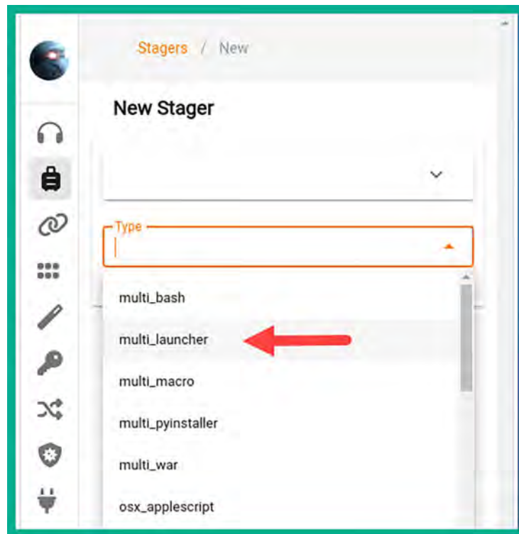
Figure 11.54: Stager types
