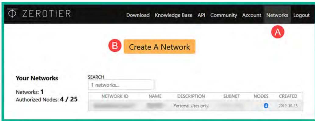
Figure 18.10: ZeroTier dashboard
