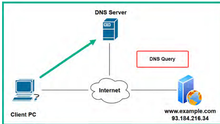
Figure 5.11: DNS query
