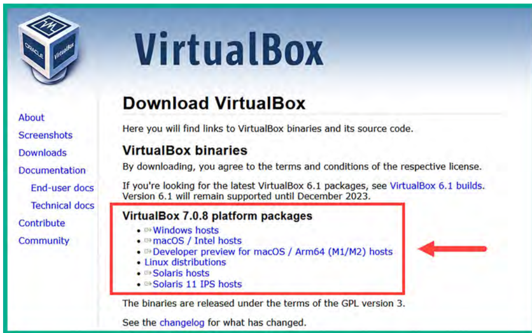
Figure 2.3: VirtualBox website
