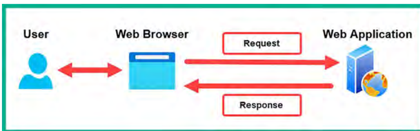
Figure 16.1: Request-response messages
