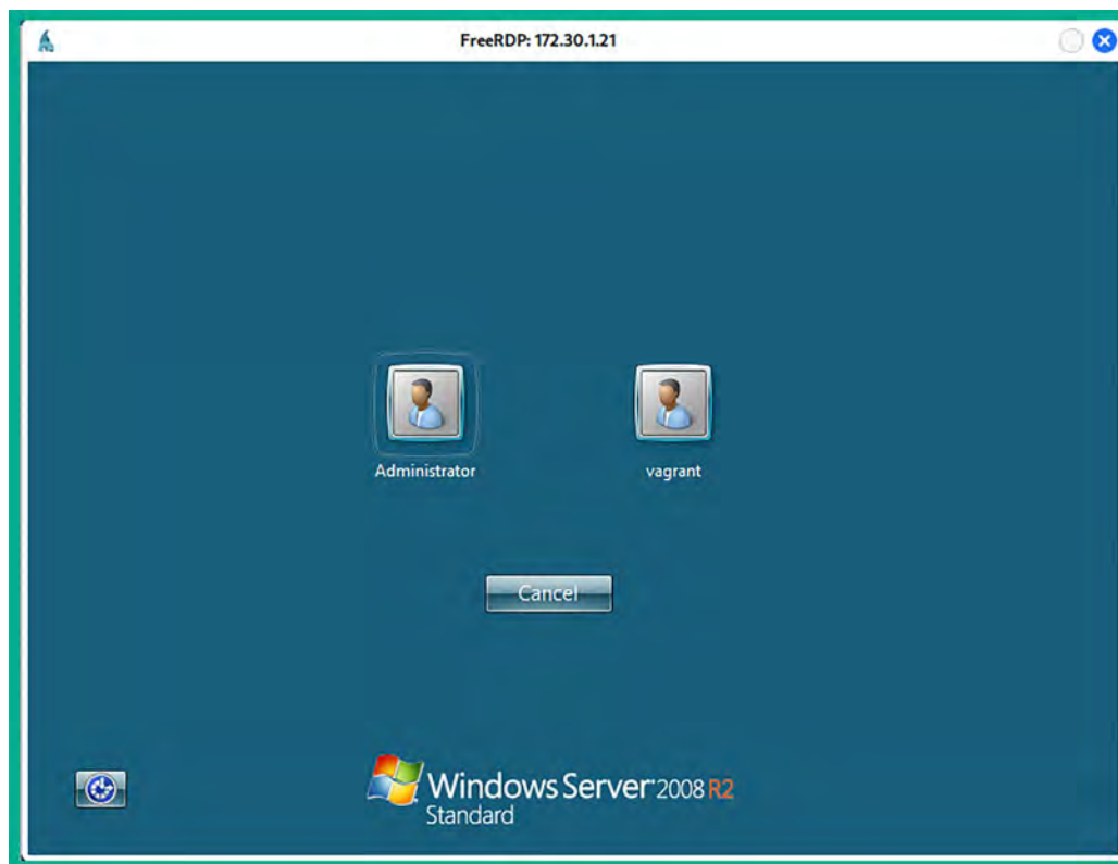
Figure 10.4: Remote Desktop
