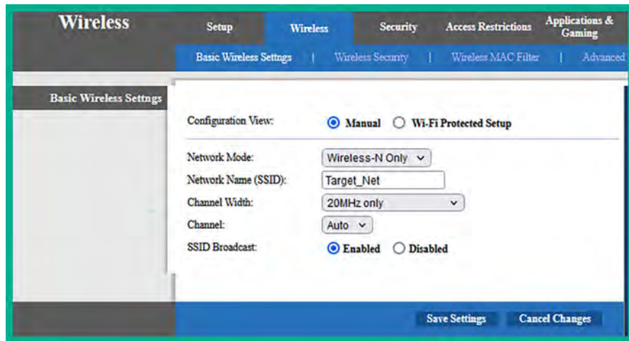
Figure 3.44: Wireless router configurations
