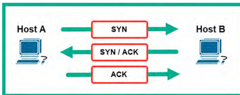
Figure 6.26: TCP 3-way handshake
