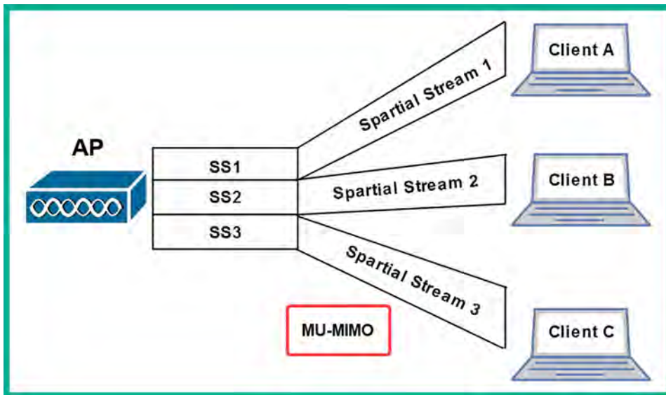
Figure 14.9: MU-MIMO operations
