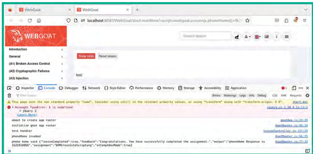
Figure 17.50: Firefox Console
