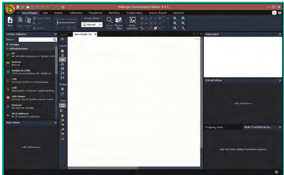
Figure 5.40: New graph
