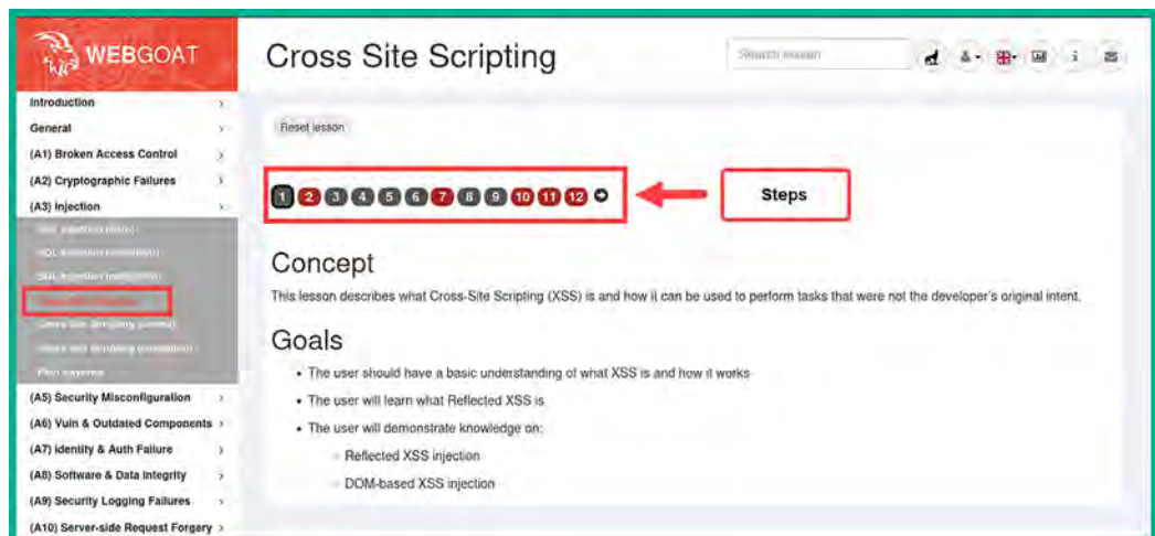
Figure 17.43: XSS exercise
