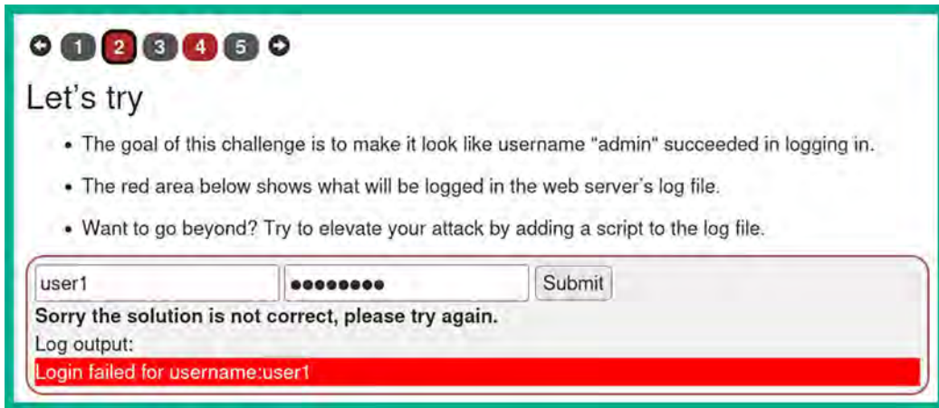
Figure 17.34: Random input
