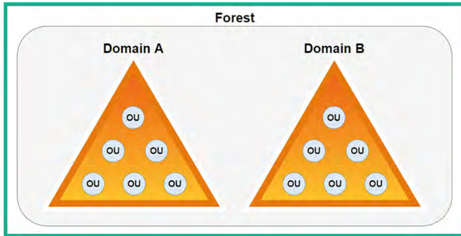
Figure 12.2: Forest structure
