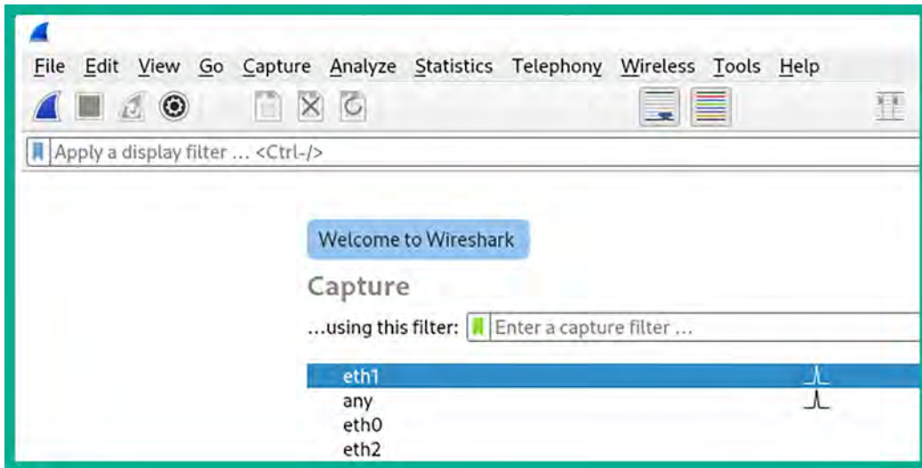
Figure 10.68: Wireshark interface
