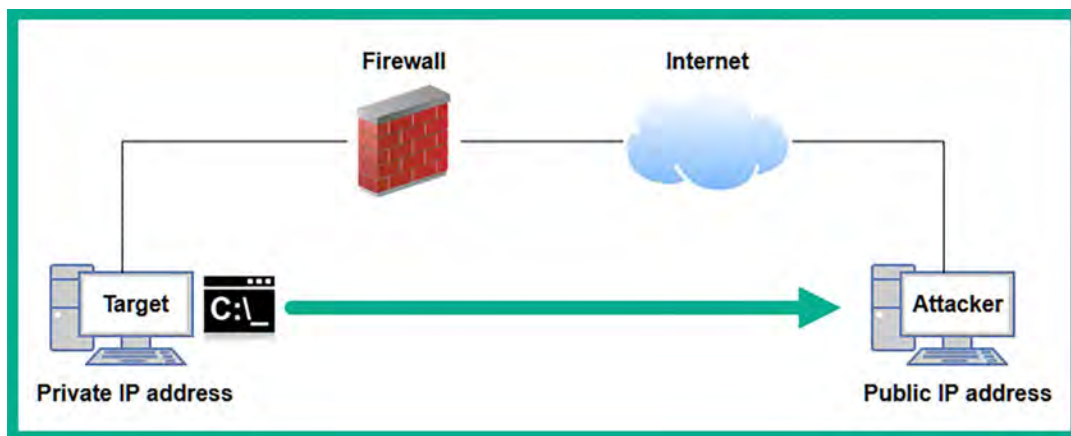
Figure 8.2: Reverse shell
