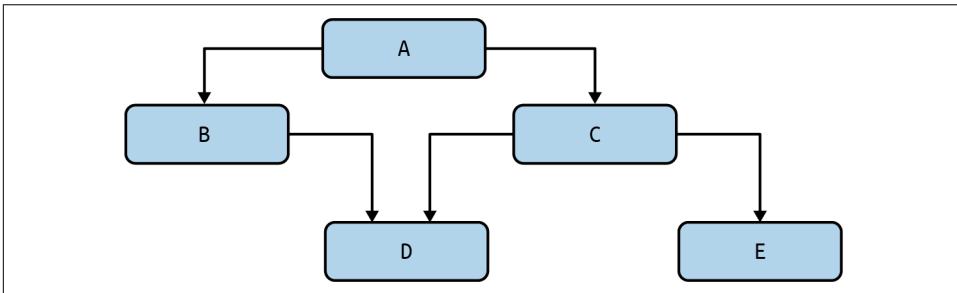
Figure 16-1. Box-and-arrows diagram
