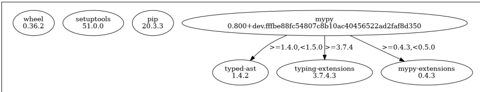
Figure 16-5. Visualizing packages
