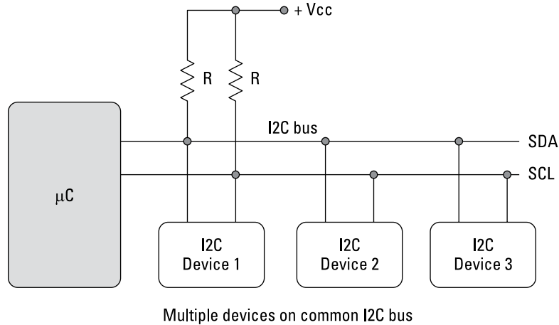
FIGURE 3-1: The I2C bus.
