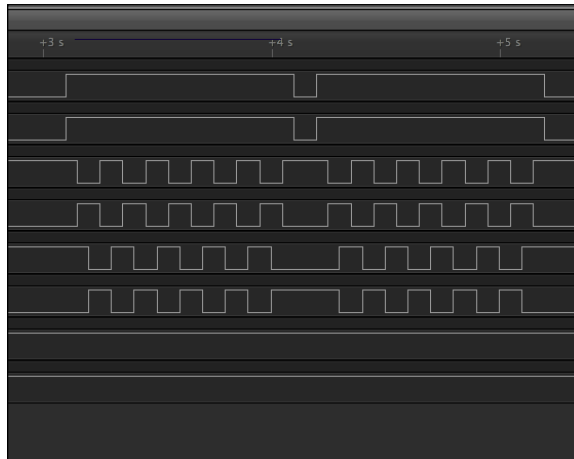
FIGURE 4-14: Logic analyzer showing the motor stepping sequence.
