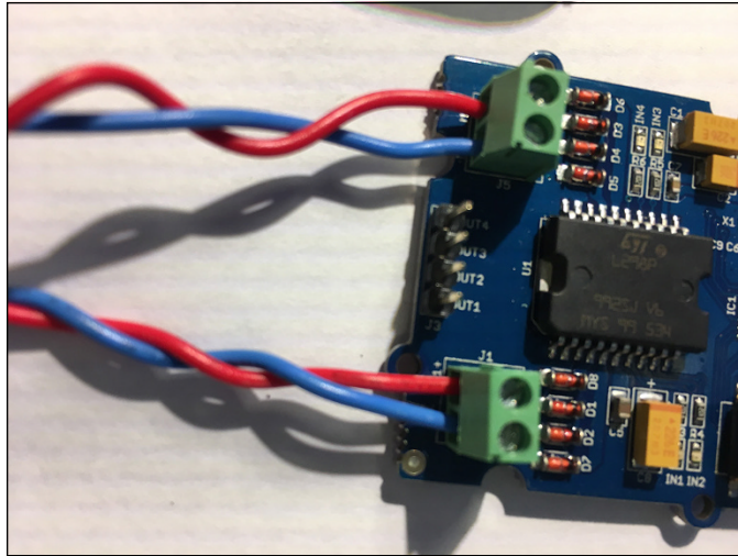
FIGURE 4-6: The wires in the I2C motor driver screw terminals.
