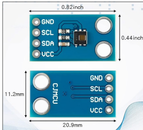
FIGURE 3-2: HDC1080 temperature and humidity sensor.
