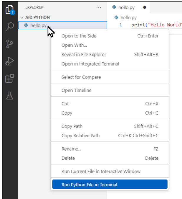
FIGURE 2-9: Run hello.py .
