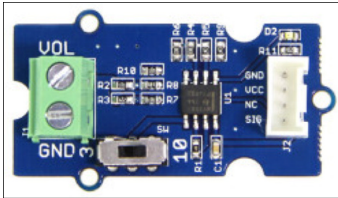
FIGURE 2-7: A Grove analog simple voltage divider.
