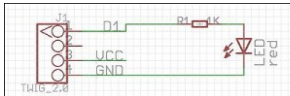
FIGURE 2-6: A simple digital Grove module with LED.
