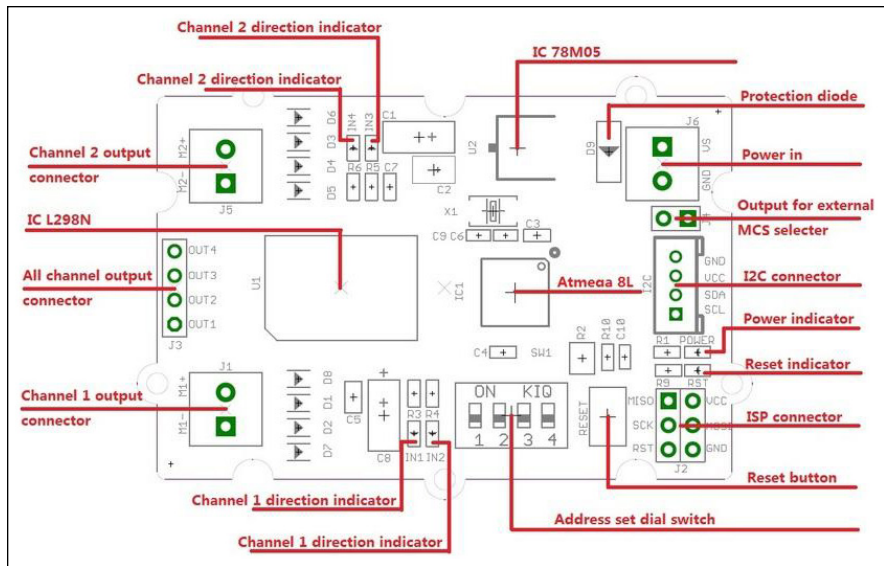
FIGURE 4-4: An annotated diagram of the I2C motor driver board.
