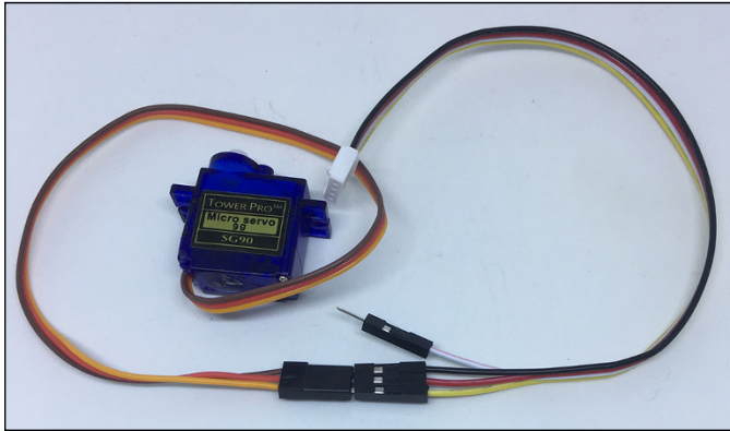
FIGURE 4-11: A servo motor correctly wired to the patch cable.
