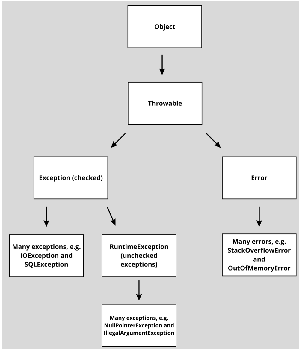
Figure 11.1 – Throwable hierarchy
