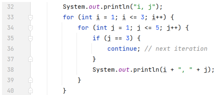
Figure 5.19 – A continue example
