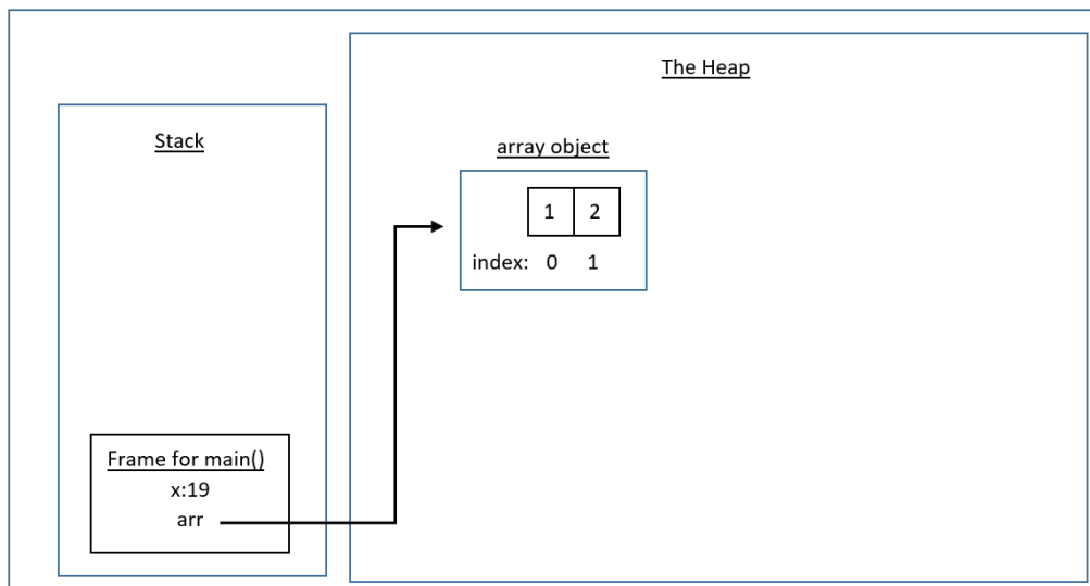
Figure 7.13 – In-memory representation of the code from Figure 7.12
