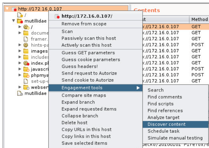
Figure 9.8: Burp Suite Discover Content Menu Item
