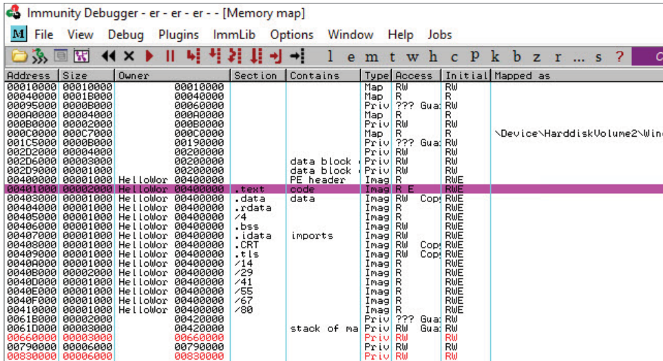
Figure 15.11: Memory Map Window
