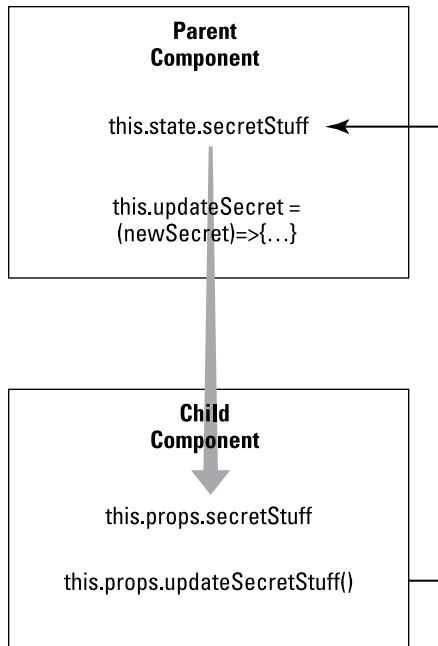
FIGURE 1-4: Pass a function to a child to do inverse data flow.
