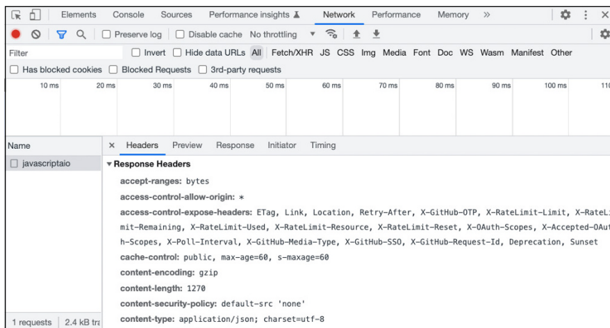
FIGURE 11-7: Viewing the HTTP headers.
