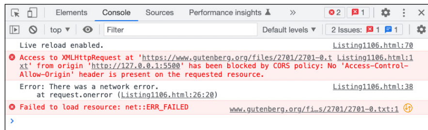
FIGURE 11-1: The error that's generated when running Listing 11-6.
