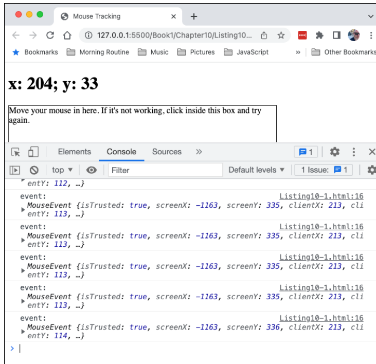
FIGURE 10-2: Viewing the event object.
