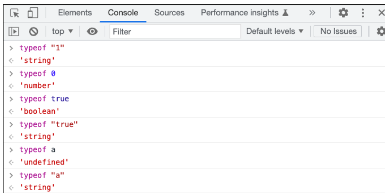
FIGURE 3-3: Using typeof to get the data type.
