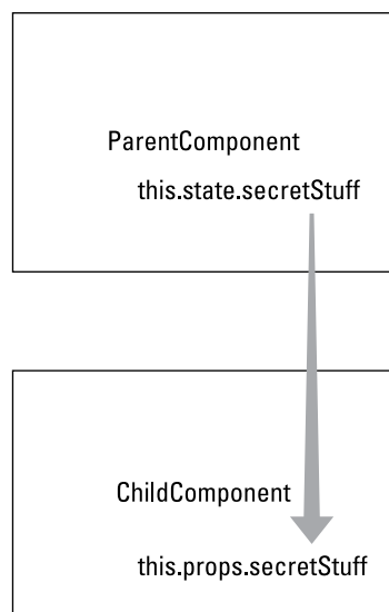
FIGURE 1-3: How state works.
