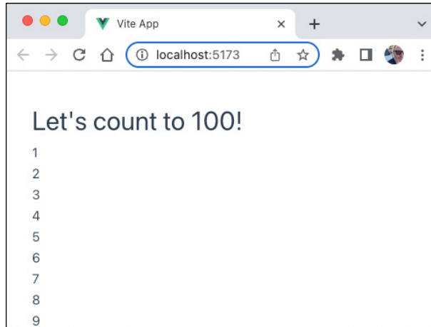
FIGURE 3-4: Counting to 100 with Vue.
