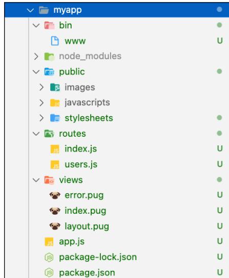
FIGURE 9-6: The default generated app's structure.
