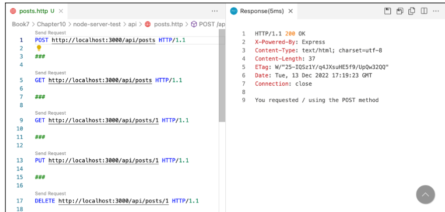
FIGURE 10-1: Testing the routes.
