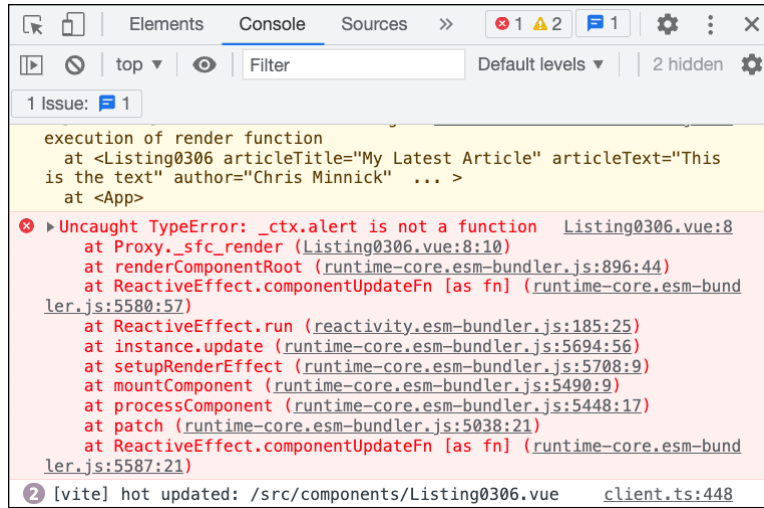
FIGURE 3-3: Templates don't have access to all JavaScript globals.
