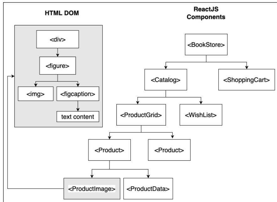
FIGURE 1-1: A React UI is a higher level of abstraction.
