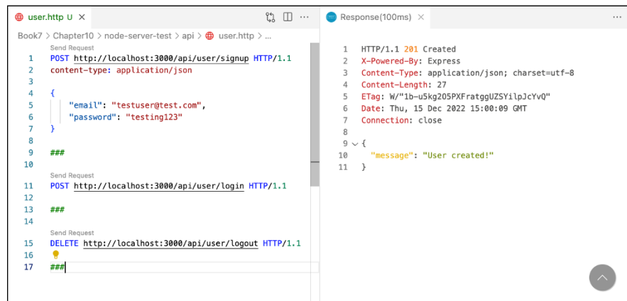
FIGURE 10-4: User created successfully.
