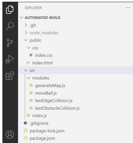
FIGURE 2-1: The reorganized project structure.
