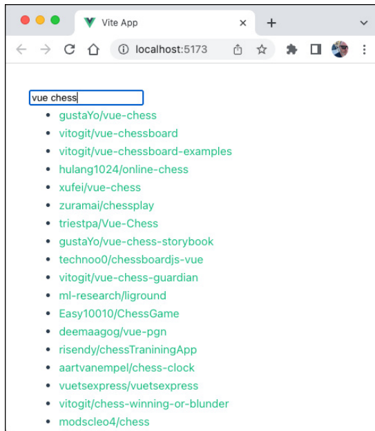
FIGURE 4-3: A dynamic search box, created using a watcher function.
