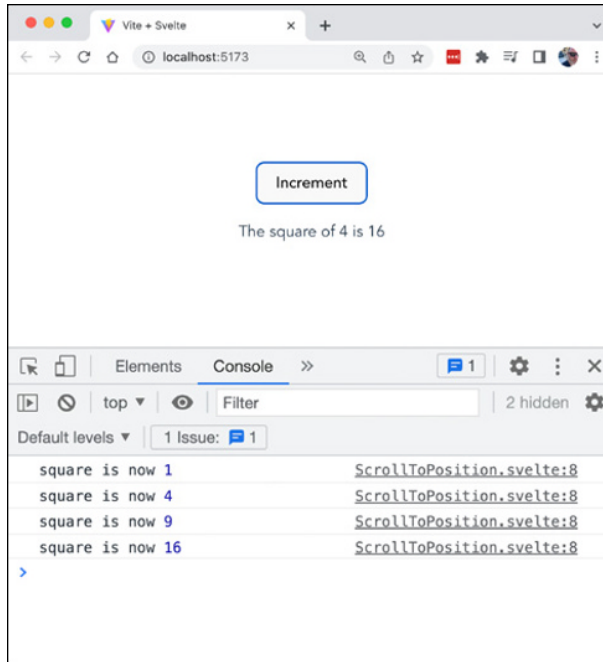
FIGURE 5-2: The values in the console and in the DOM match now.
