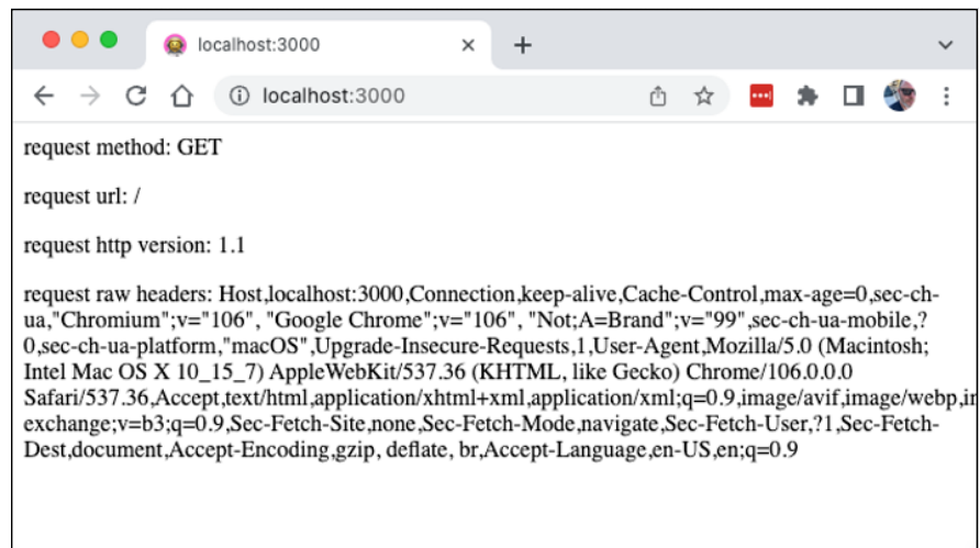
FIGURE 5-1: Viewing your request headers.
