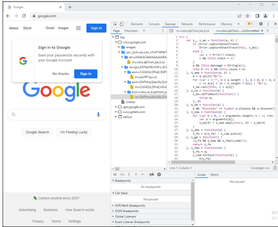
FIGURE 1-9: Google.com's JavaScript, prettified.
