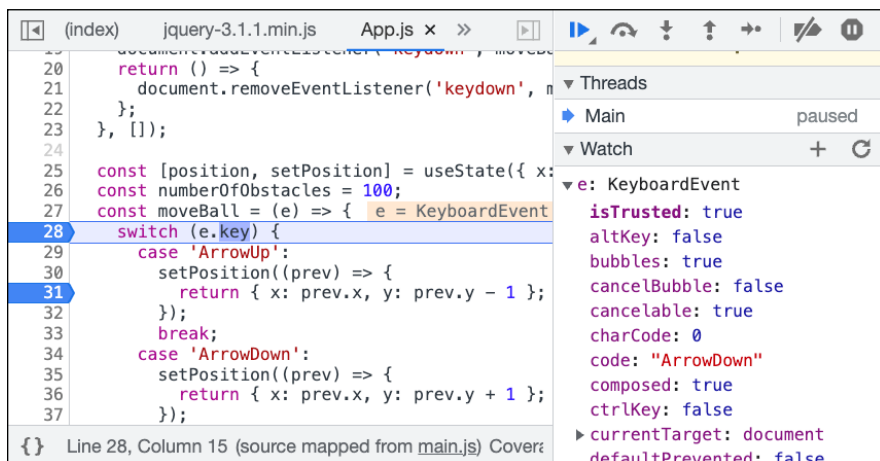
FIGURE 3-6: Setting a watch expression.
