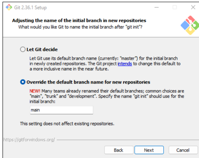
FIGURE 2-12: Setting the default branch name.
