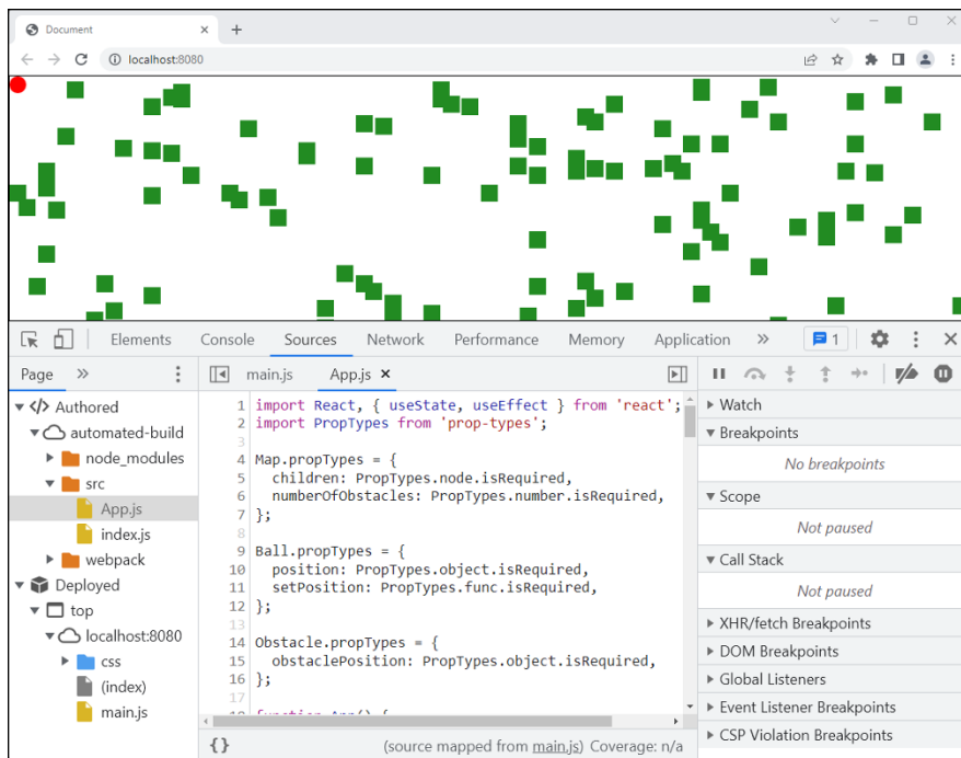
FIGURE 3-4: Viewing your source code in the Sources panel.
