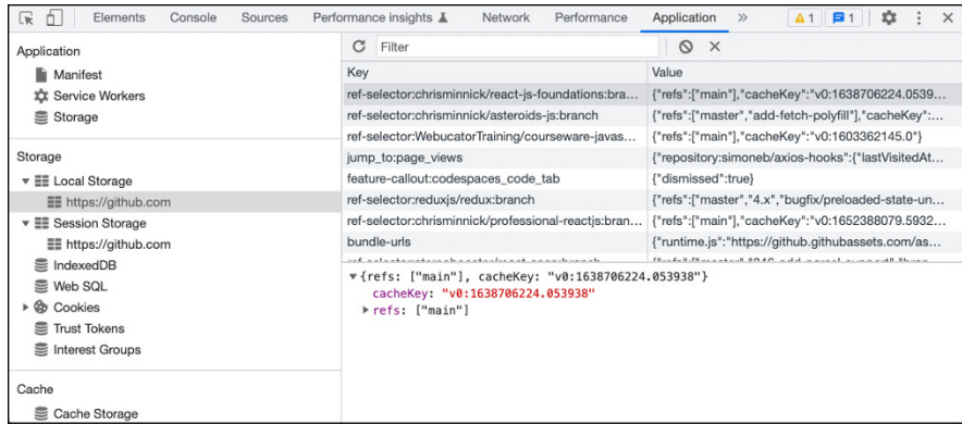
FIGURE 1-4: Viewing local data storage on the Application tab.
