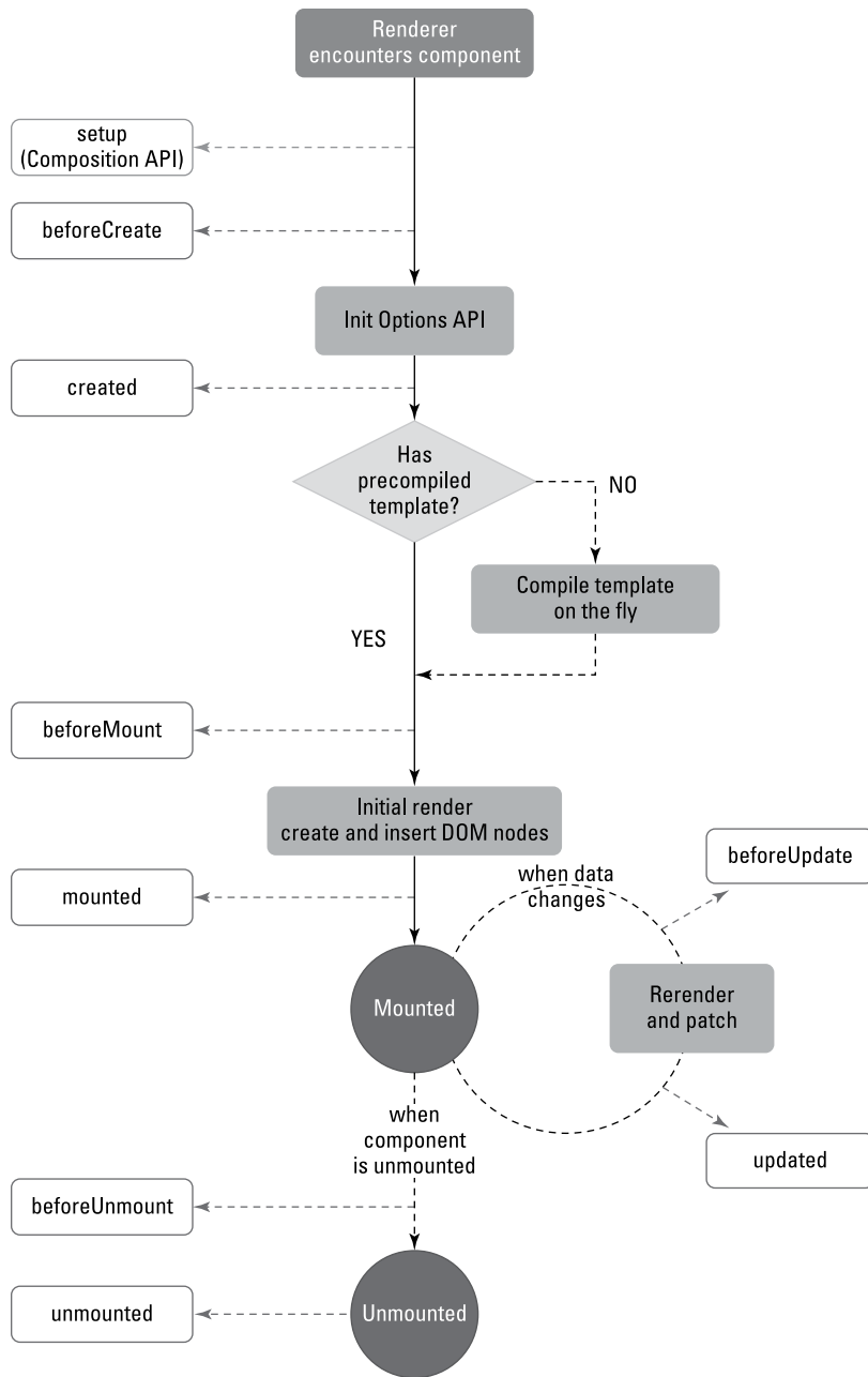
FIGURE 2-1: The Vue component instance lifecycle.
