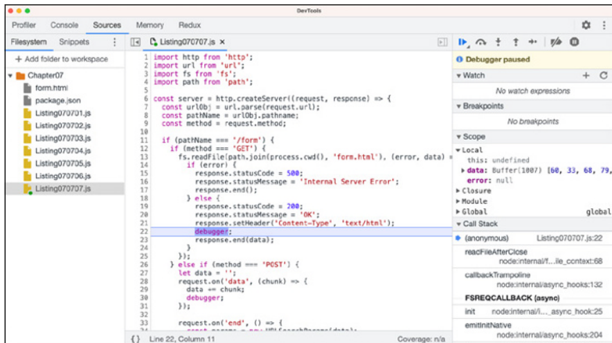
FIGURE 7-13: The paused debugger.
