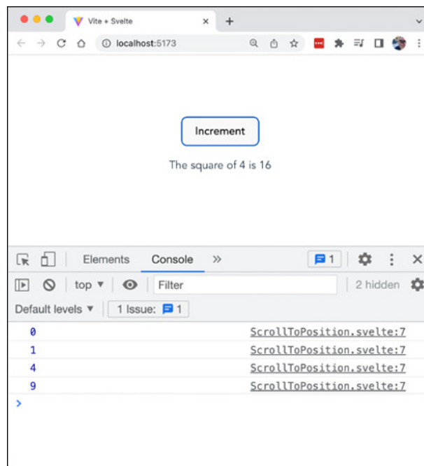
FIGURE 5-1: The console. log() method receives the old value.
