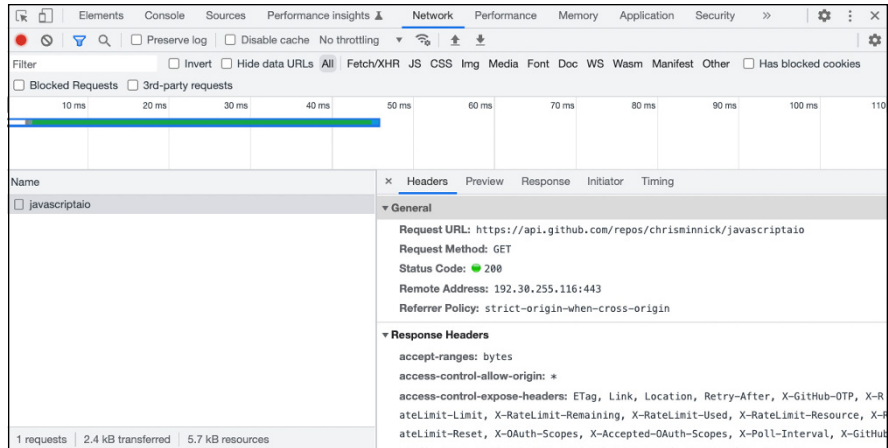
FIGURE 11-6: The Network tab.
