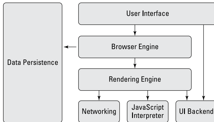
FIGURE 1-1: The components of a web browser.
