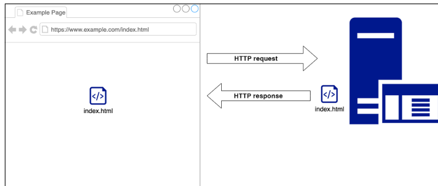
FIGURE 1-4: HTTP request and response.
