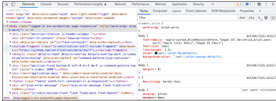
FIGURE 1-2: The Elements tab contains tools for inspecting the DOM, CSSOM, and layout.
