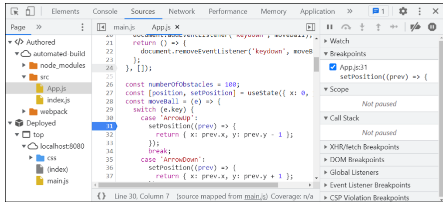
FIGURE 3-5: Setting a breakpoint.
