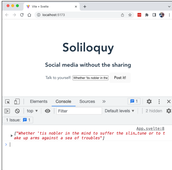
FIGURE 2-2: Array methods don't trigger reactivity.
