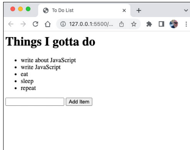
FIGURE 2-4: A simple to-do list, created using DOM methods.
