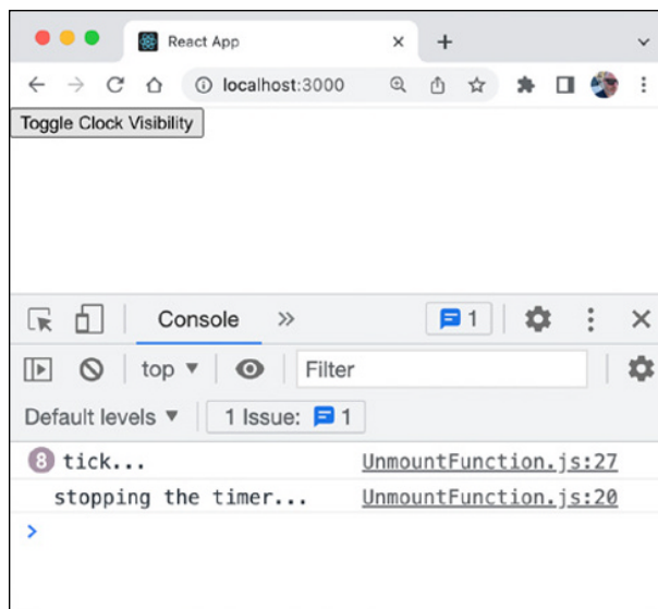
FIGURE 3-3: Returning a function to stop the clock.
