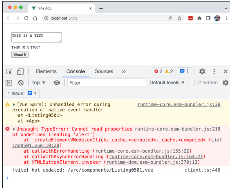
FIGURE 5-3: Access to globals is restricted in inline event handlers.
