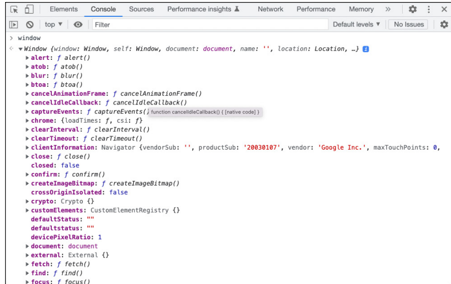
FIGURE 2-2: Viewing the properties of the window object.
