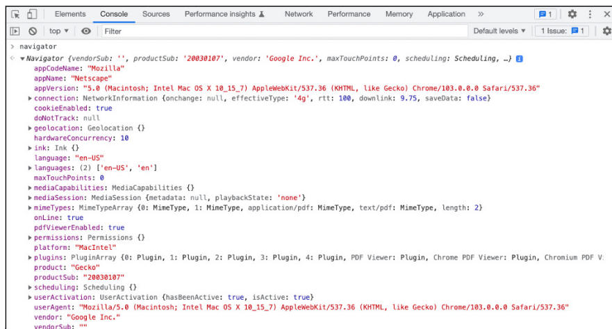
FIGURE 2-1: Viewing the properties and methods of the navigator object.
