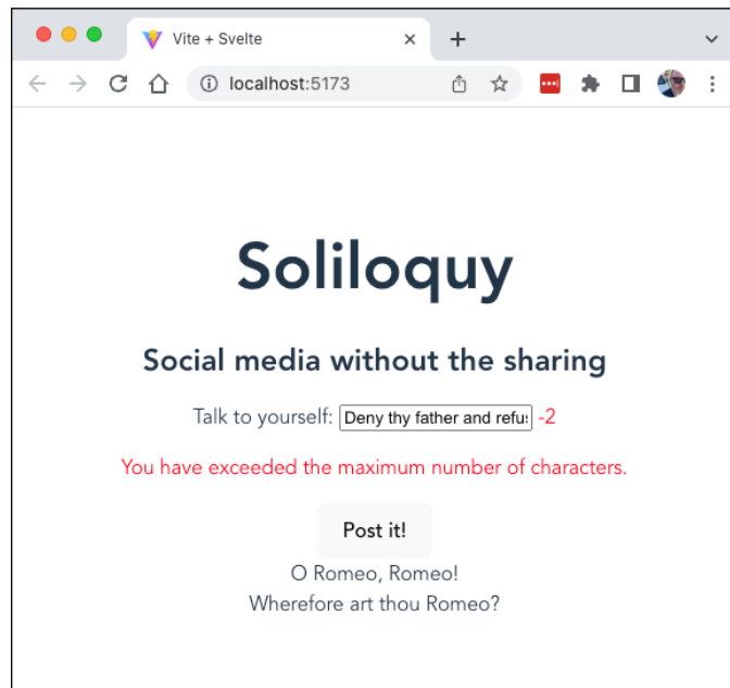
FIGURE 2-4: The Soliloquy app, with character counting and an error message.
