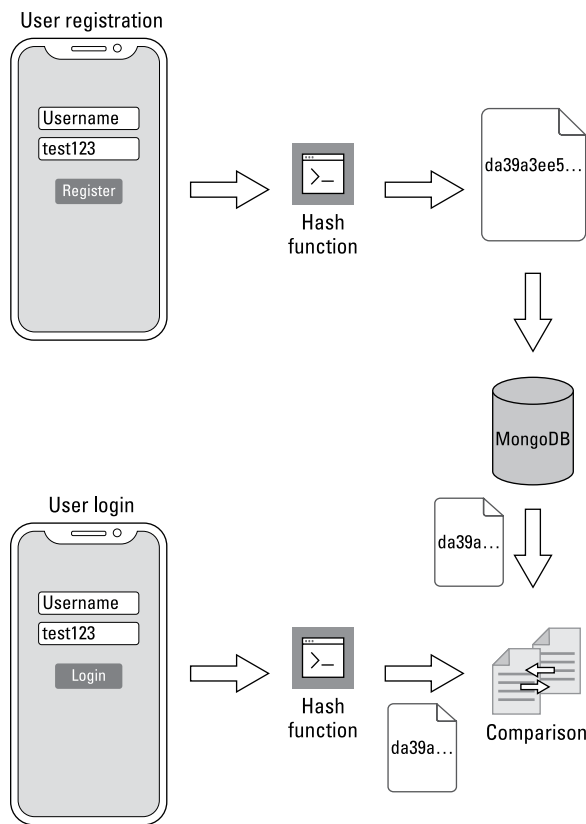
FIGURE 10-3: Using a one-way hash.
