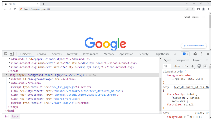
FIGURE 1-6: Viewing the code at Google.com.
