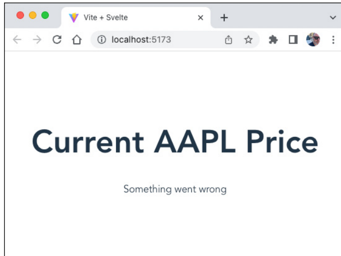
FIGURE 5-4: Displaying an error message when a Promise is rejected.
