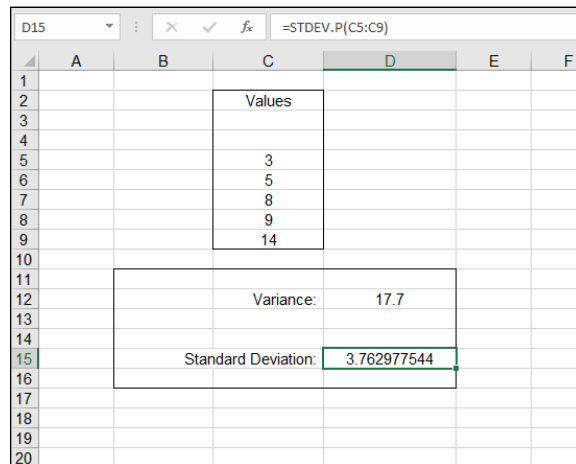
FIGURE 9-6: Calculating the standard deviation.
