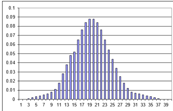
FIGURE 11-9: A Poisson distribution with a mean of 20.
