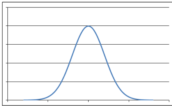
FIGURE 9-7: Displaying a normal distribution in a graph.
