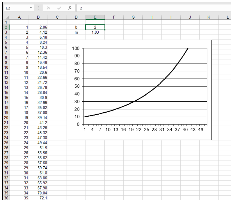
FIGURE 11-1: An exponential curve.
