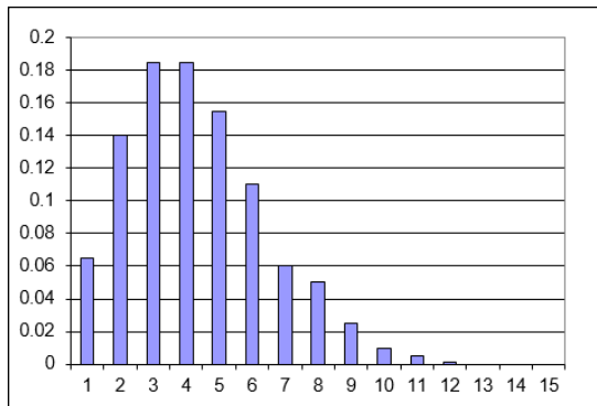
FIGURE 11-10: A Poisson distribution with a mean of 4.
