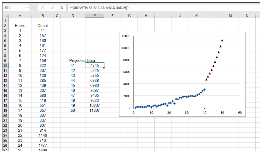
FIGURE 11-7: Demonstrating use of the GROWTH function to project exponential data.
