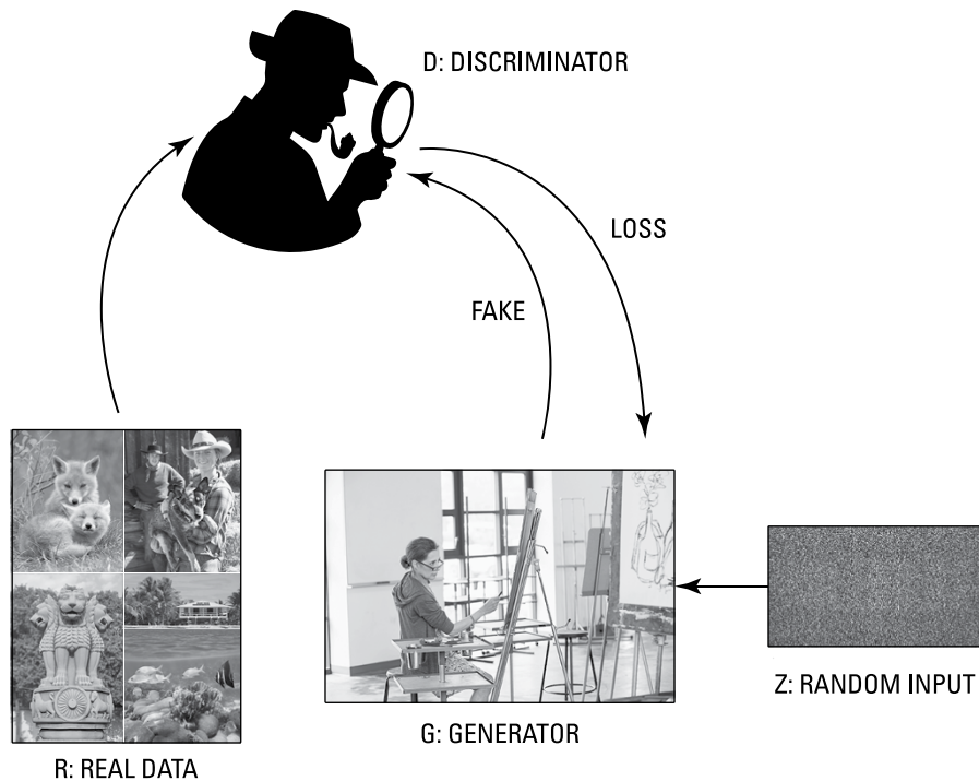
FIGURE 11-6: How a GAN network works, oscillating between generator and discriminator.
