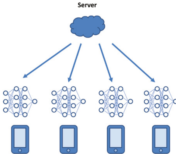
Figure 5.13: The federated learning architecture
