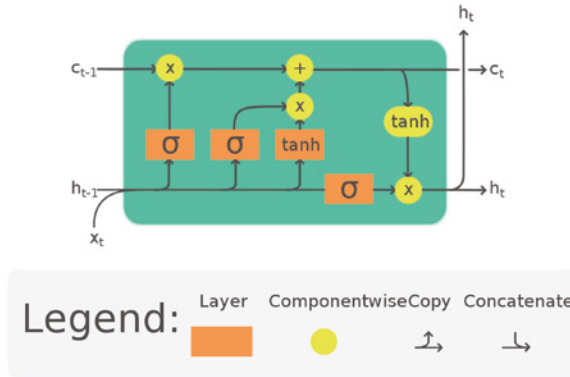
Figure 4.36: The long short memory unit structure
