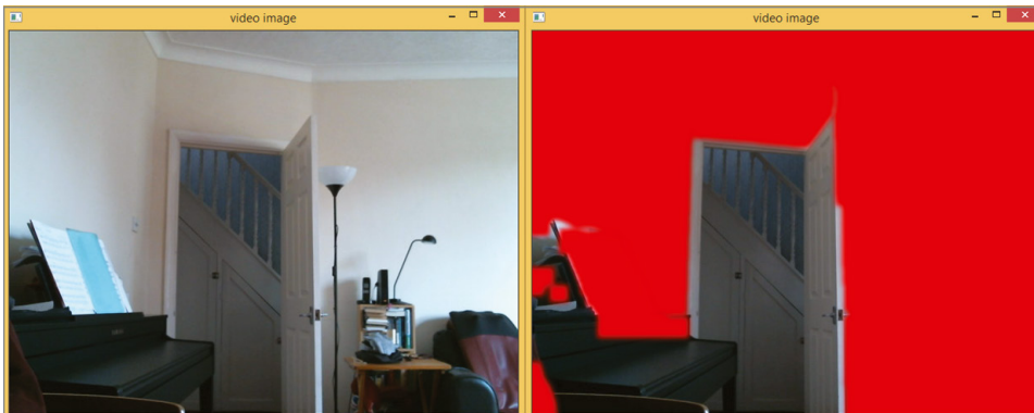
Figure 7.35: The original webcam image (left) and the image with background removed, shown in red (right)
