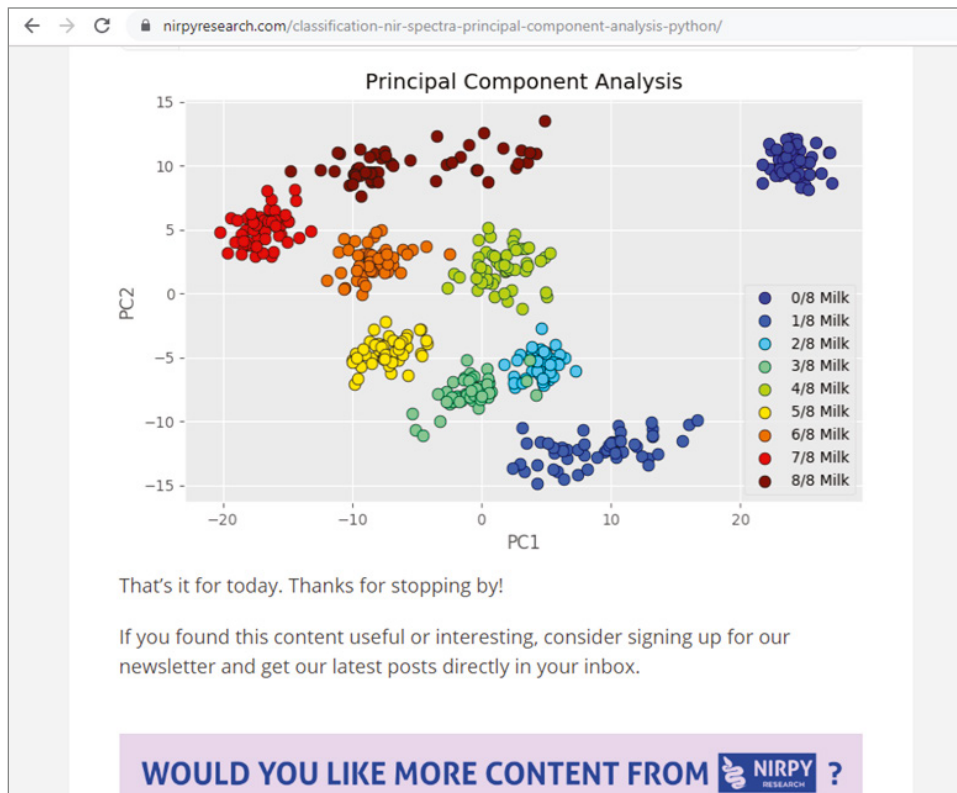
Figure 11.10: The milk powder spectral data classification with PCA.
