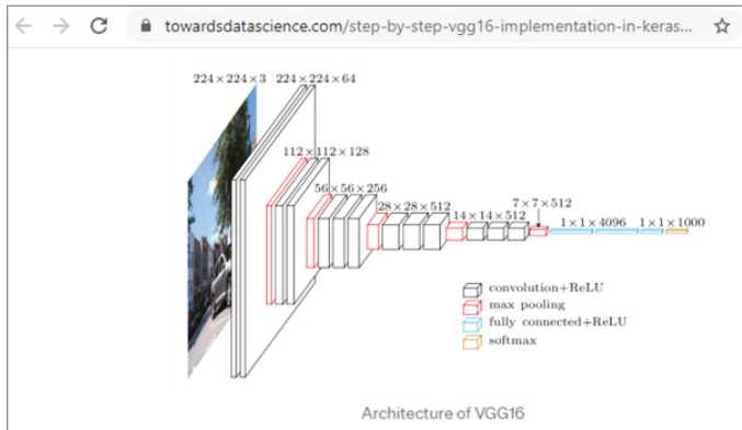
Figure 4.13: The architecture of VGG16 neural networks
