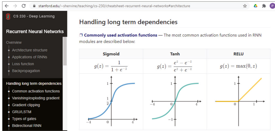
Figure 4.9: Commonly used activation functions
