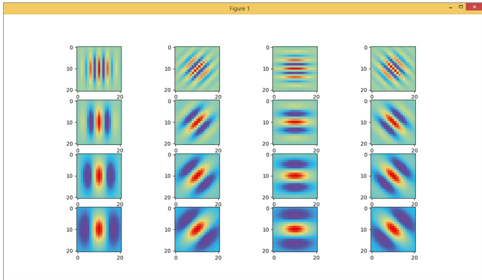
Figure 5.28: The wavelets of the Gabor filters at four different wavelengths (rows) and four different orientations (columns)
