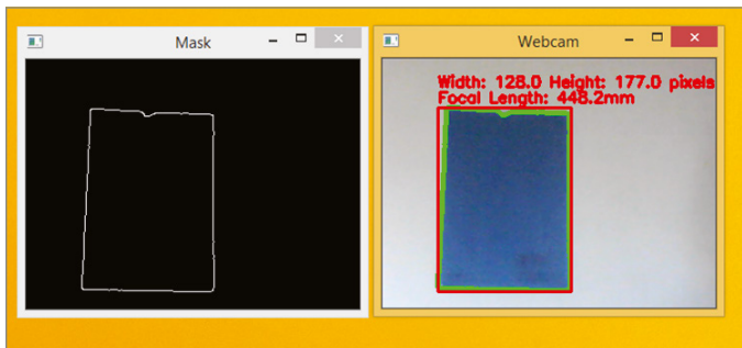
Figure 7.16: The detected A4 paper mask (left), the A4 paper width and height in pixels, and the calculated focal length in mm (right)
