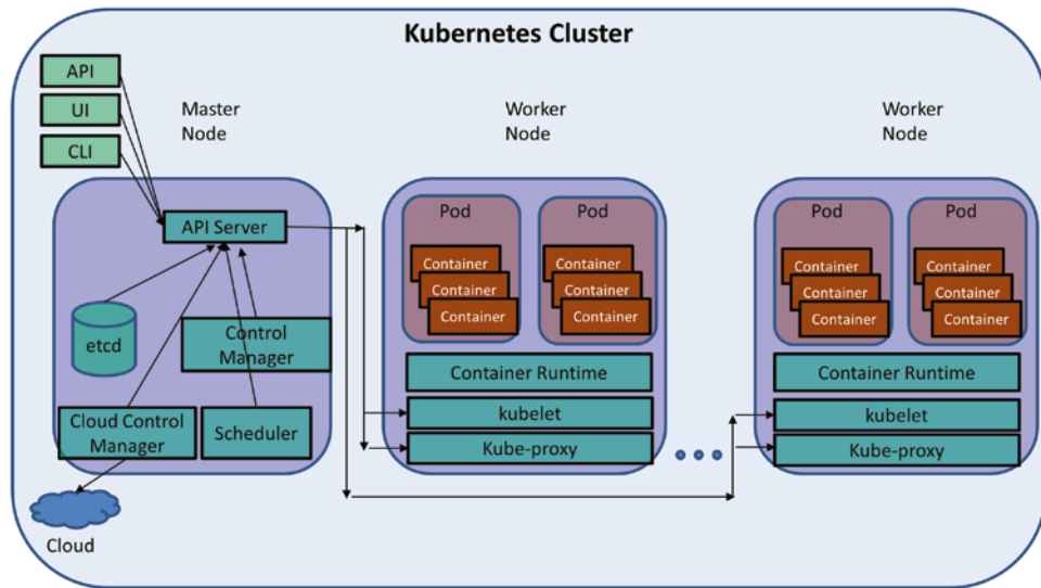
Figure 12.11: The schematic diagram of the Kubernetes architecture
