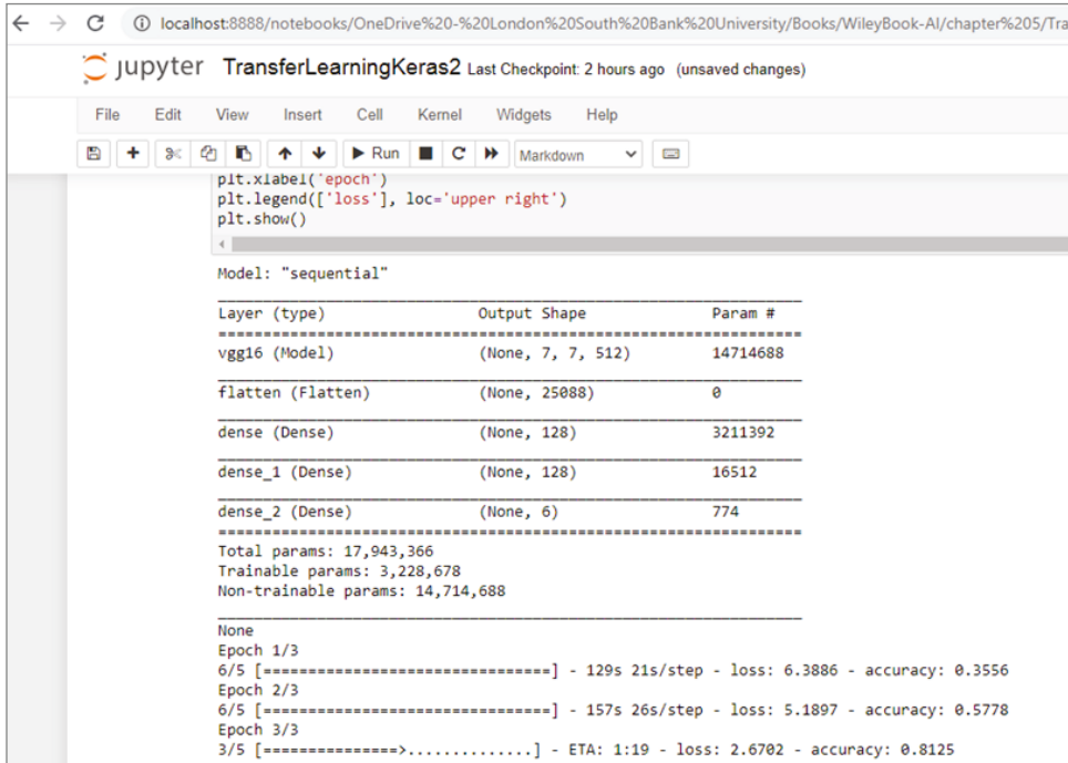
Figure 5.8: The model structure and the model training output
