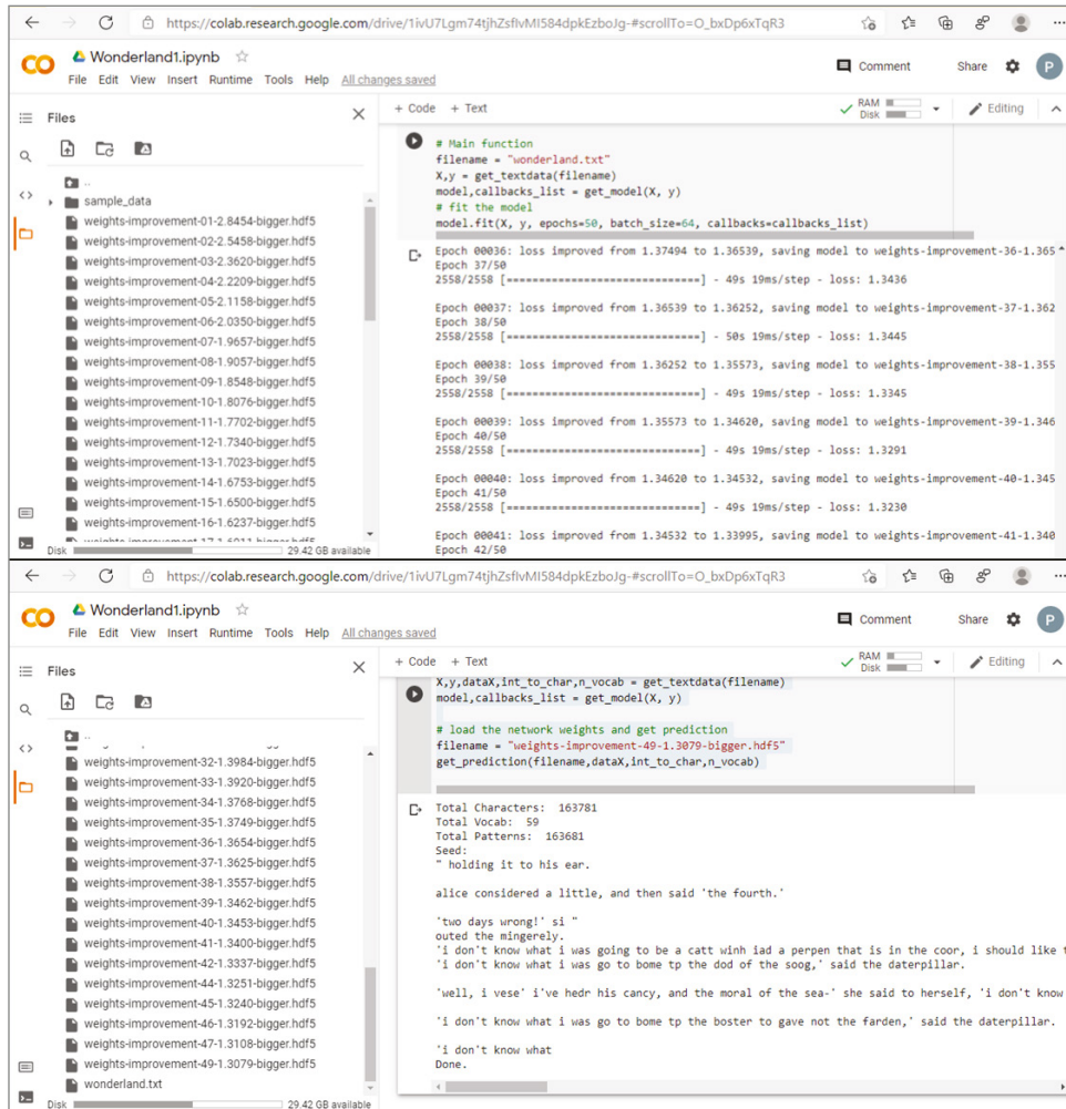
Figure 10.2: The training of the LSTM model for the Alice in Wonderland text (top) and using the trained model for text generation (bottom)
