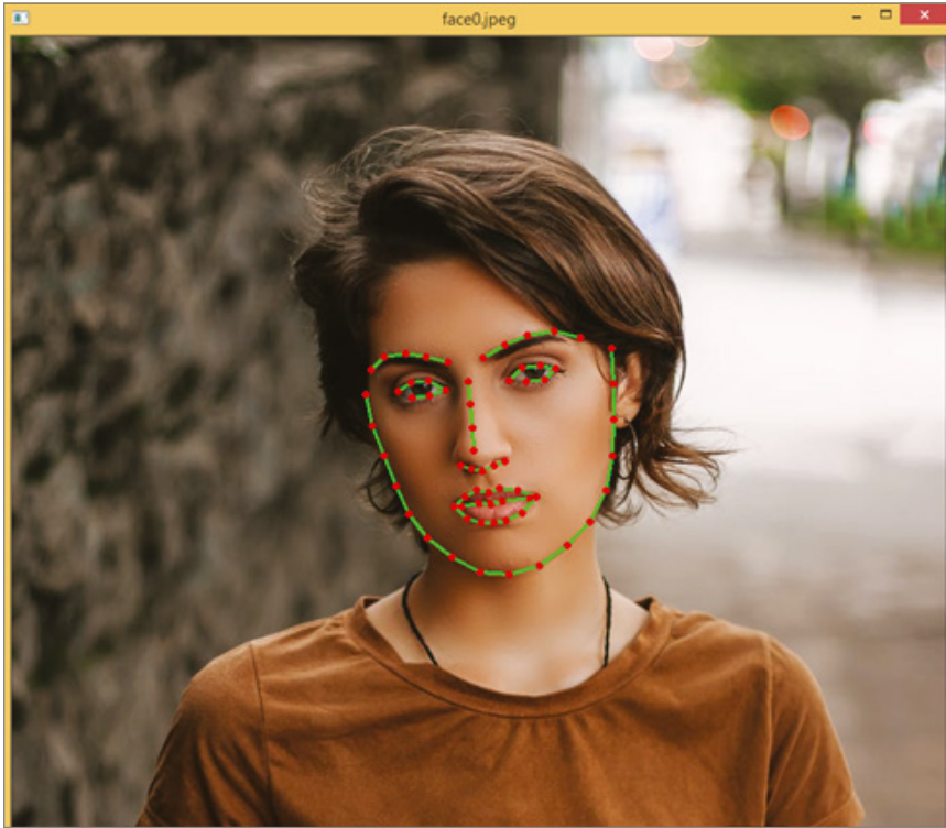
Figure 6.18: The first face image from the face0 . jpeg file
