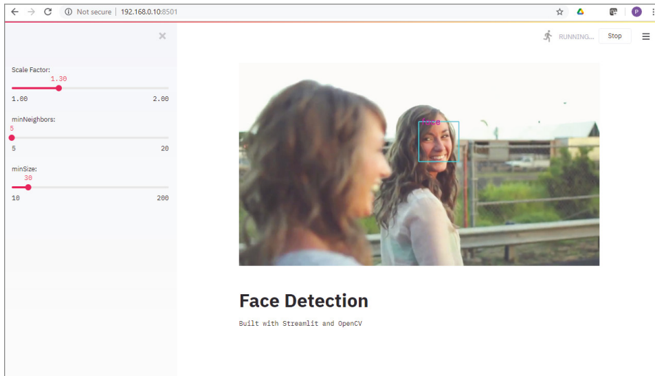
Figure 6.23: The output of the StreamlitWebcamFace.py program, which shows the three sliders for adjusting the scaleFactor , minNeighbors , and minSize parameters, and with a face detected in the image
