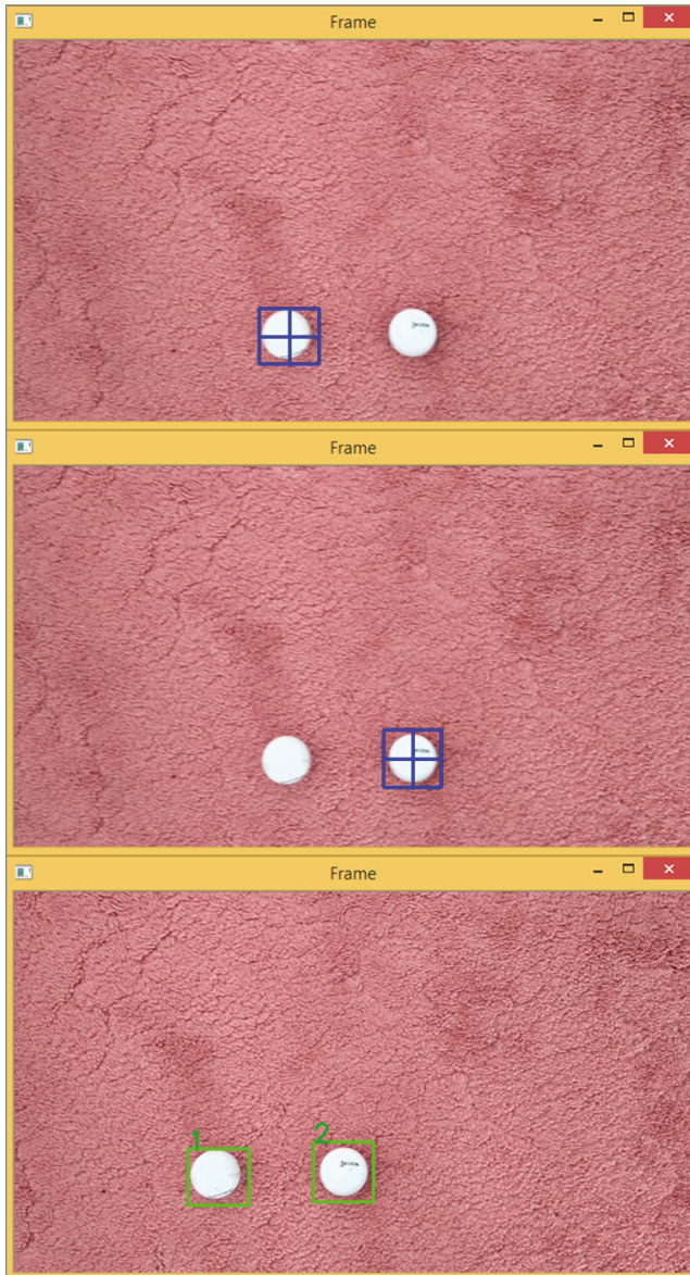
Figure 7.19: The multiple objects tracking through a webcam. Two golf balls were selected (top and middle) and were tracked (bottom).
