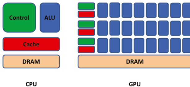
Figure 12.1: The CPU and GPU architectures where GPU has a vast number of ALUs
