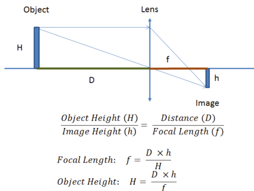
Figure 7.15: The simple camera imaging system and the relationships between object height ( H ), object distance ( D ), image height ( h ), and focal length ( f ).
