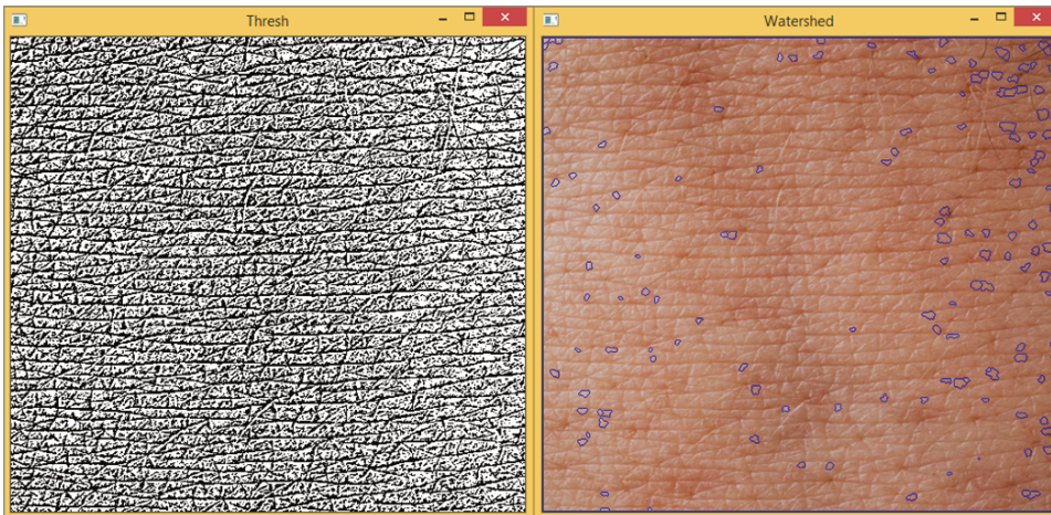
Figure 7.26: The Gaussian threshold (left) and segmented image (right) by using OpenCV watershed image segmentation
