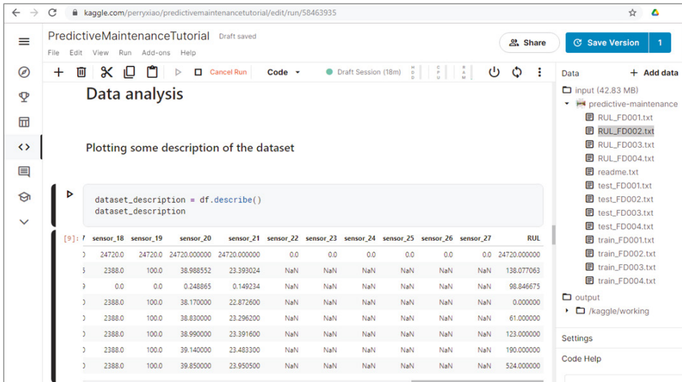
Figure 11.19: The last few columns of the dataset with the RUL column added at the end.
