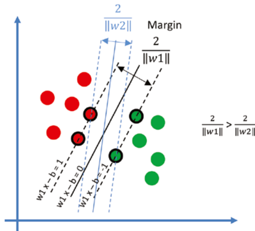
Figure 3.1: The support vector machine with two sets of data points, the hyperplane (solid line), the margin (between two dashed lines), and the support vectors (circled points on the dashed line)
