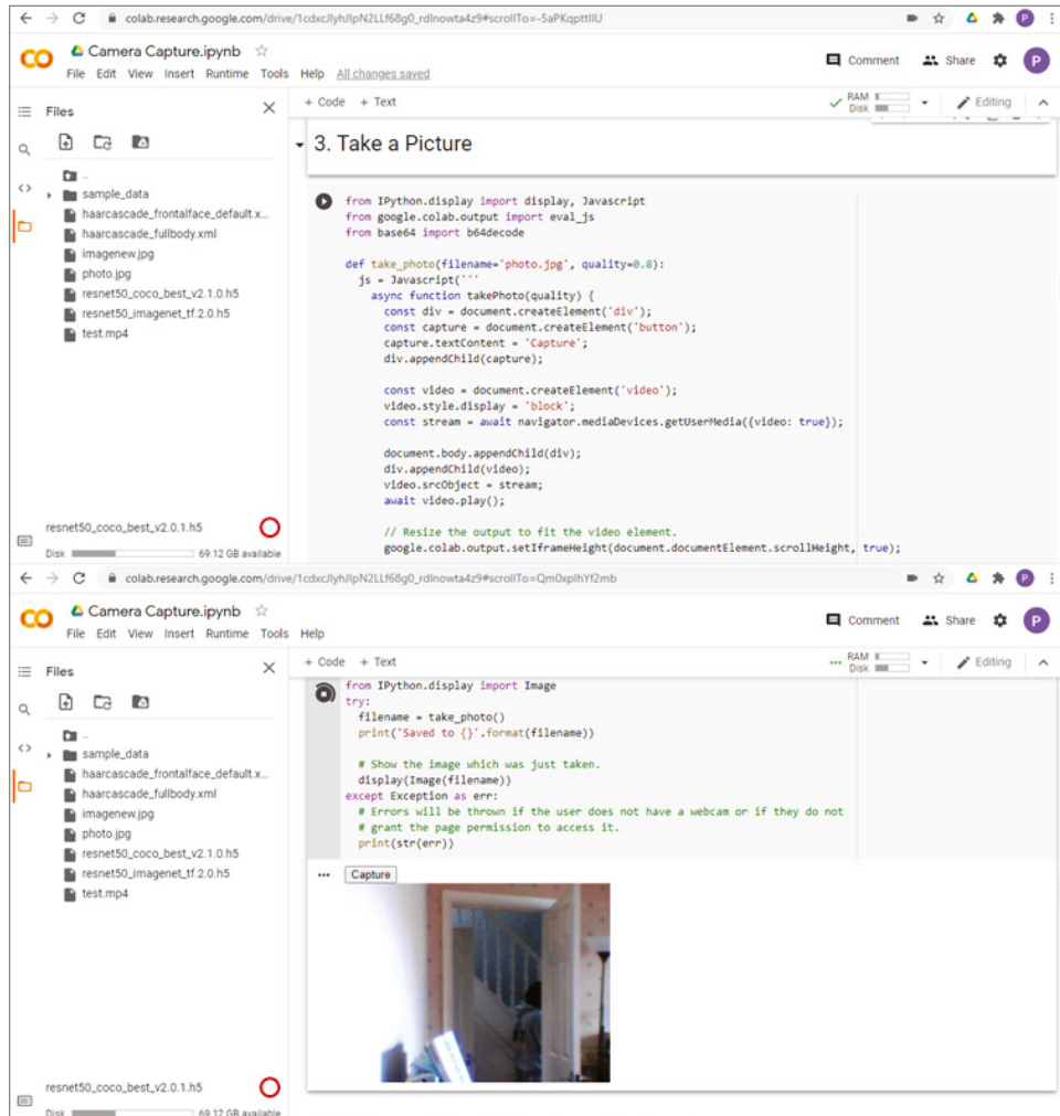
Figure 7.7: The Section 3 code to capture an image from a webcam (top) and the image captured (bottom)
