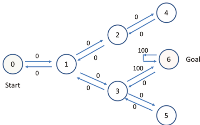
Figure 3.19: A simple routing problem with seven states, with 0 as the start state and 6 as the goal state
