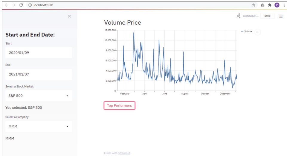
Figure 11.13: The web page output of the Streamlit stock price web app example.
