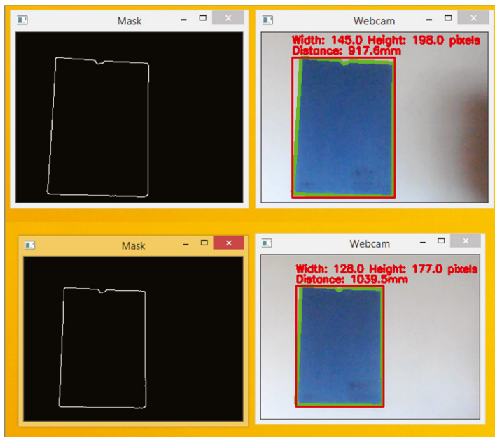
Figure 7.17: The detected A4 paper mask (left), the A4 paper width and height in pixels, and the calculated distance of A4 paper to the webcam in mm (right)
