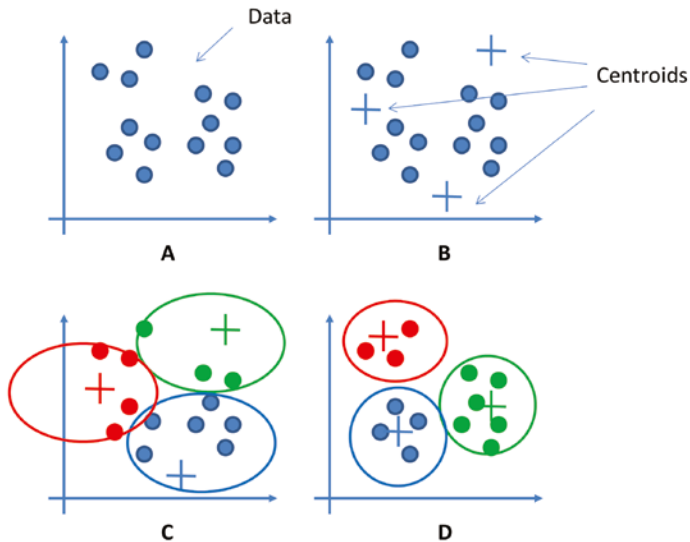
Figure 3.17: The steps of K-means clustering
