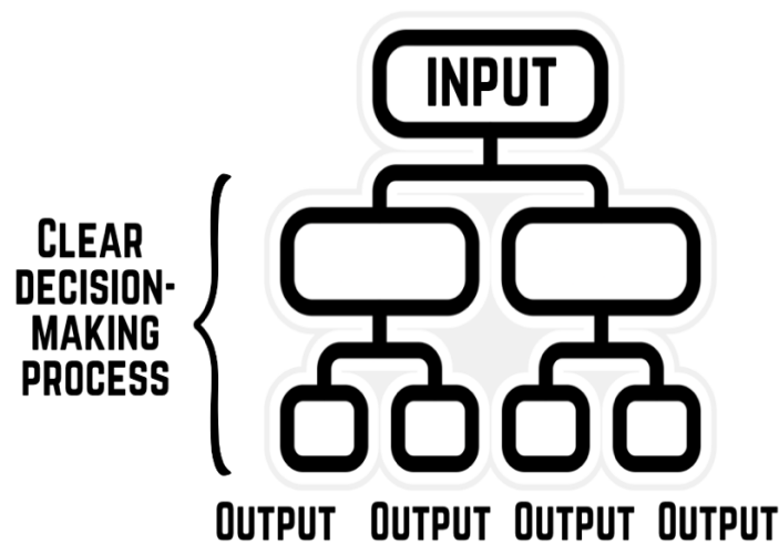
Figure 1: Decision tree
