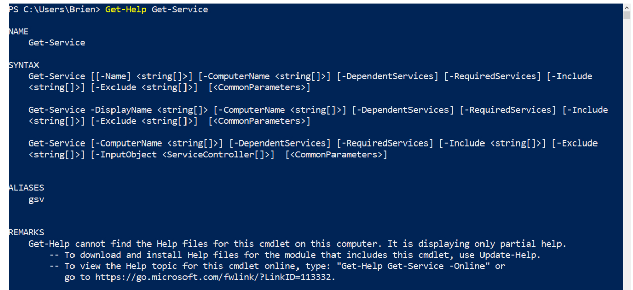
Figure 5: Use Get-Help for help using any PowerShell cmdlet.
